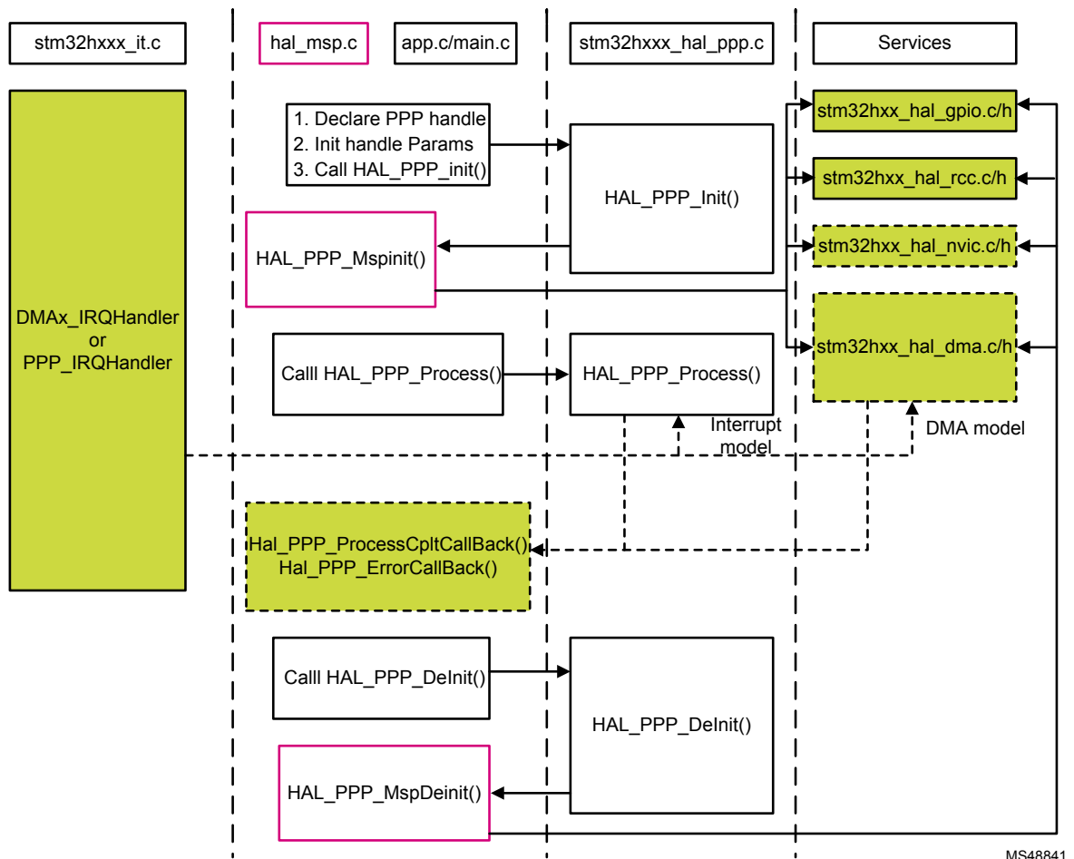
Figure 9. HAL driver model
