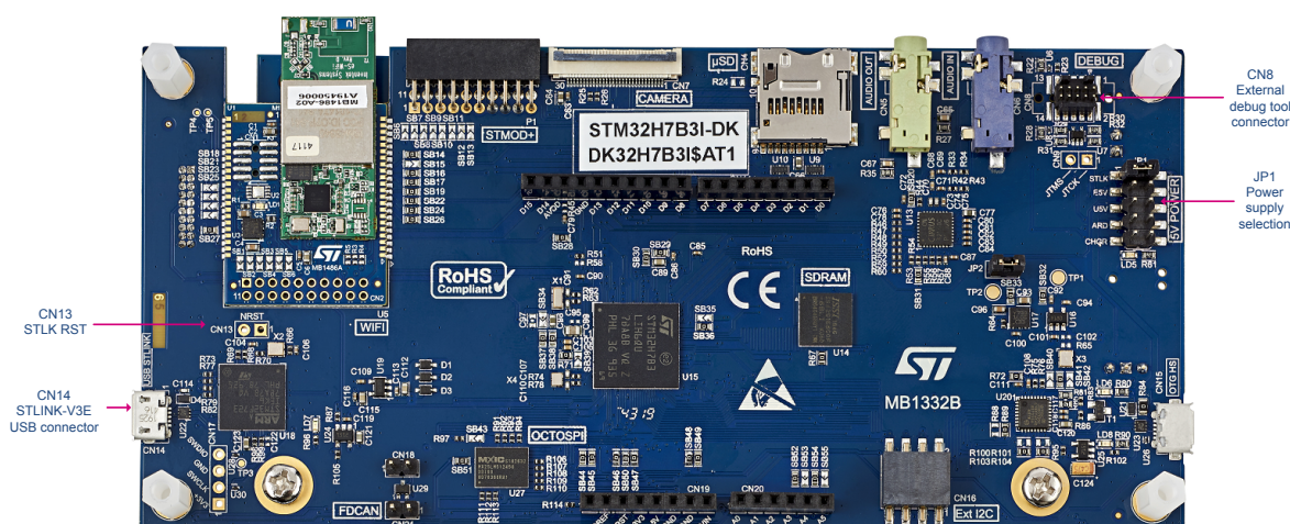
Figure 9. Connecting an external debug tool to program the onboard STM32H7B3I-DK
