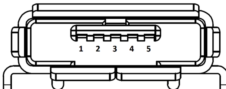
Figure 17. CN15 USB OTG HS Micro-AB connector (Front view)
