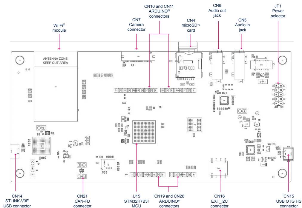
Figure 5. STM32H7B3I-DK PCB layout (bottom view)
