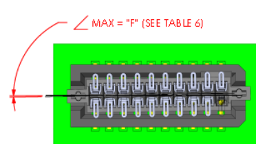
FINAL Z AXIS ANGULAR MISALIGNMENT
