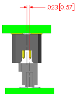
INITIAL Y AXIS LINEAR MISALIGNMENT
