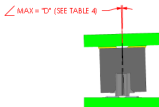
FINAL X AXIS ANGULAR MISALIGNMENT
