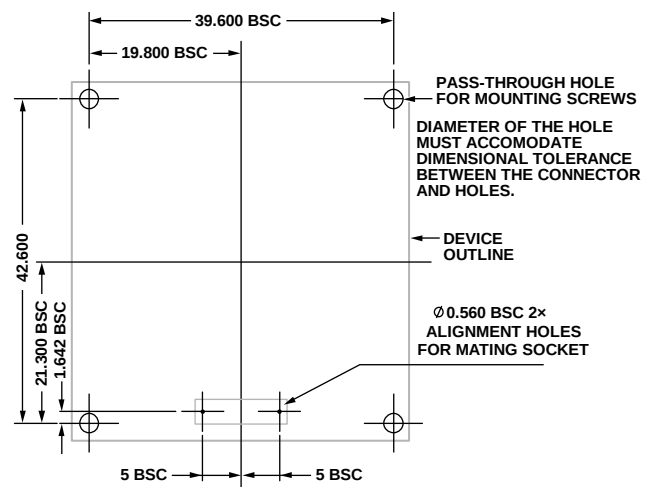
Figure 26. Mounting Example
