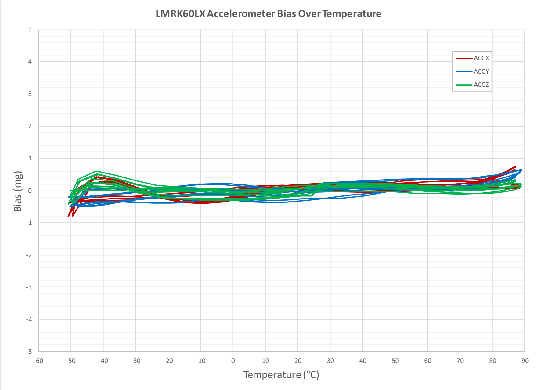
Normalized accelerometer bias over calibrated temperature range
