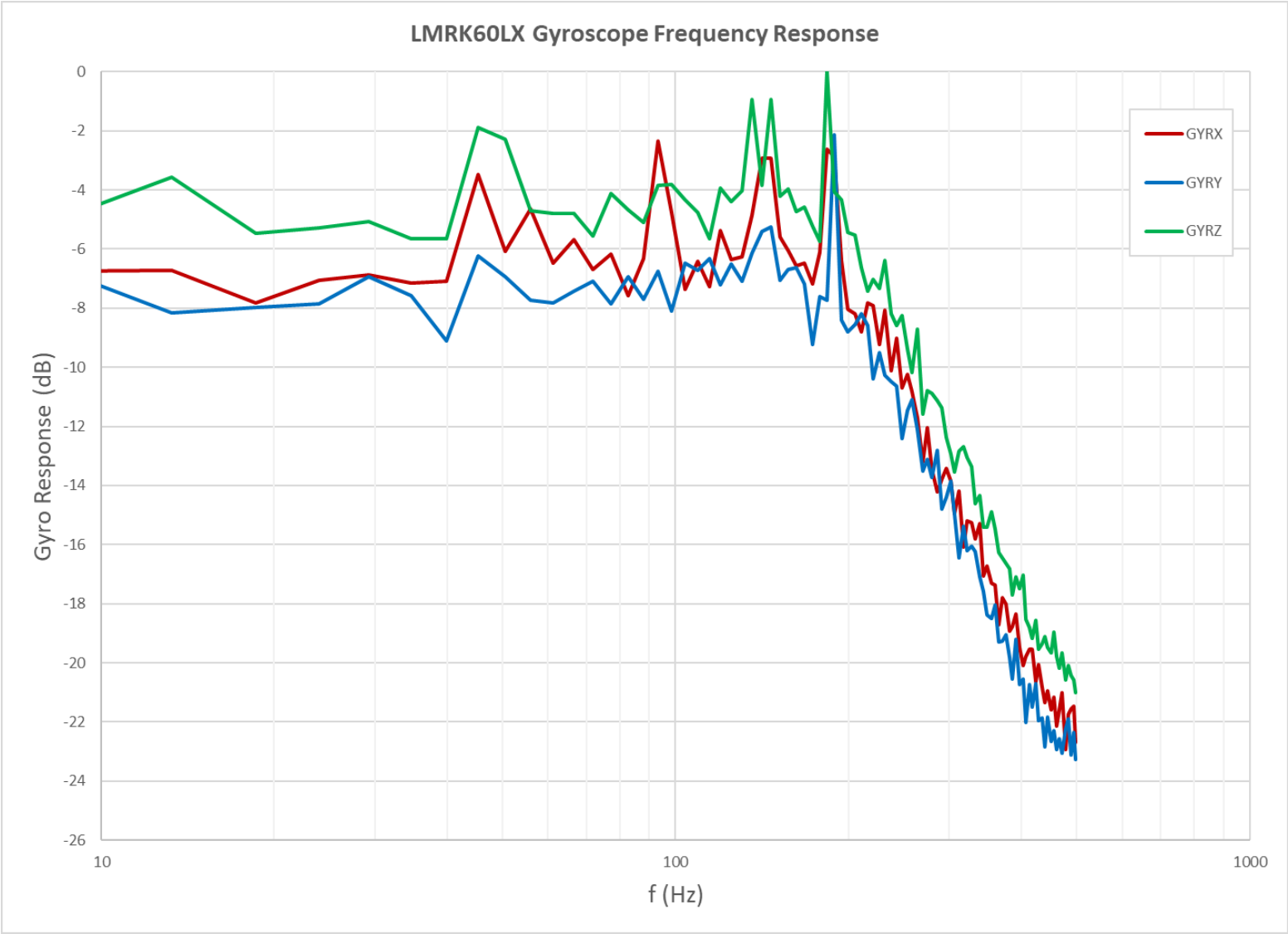
Gyroscope frequency response with LPF set to 250 Hz
