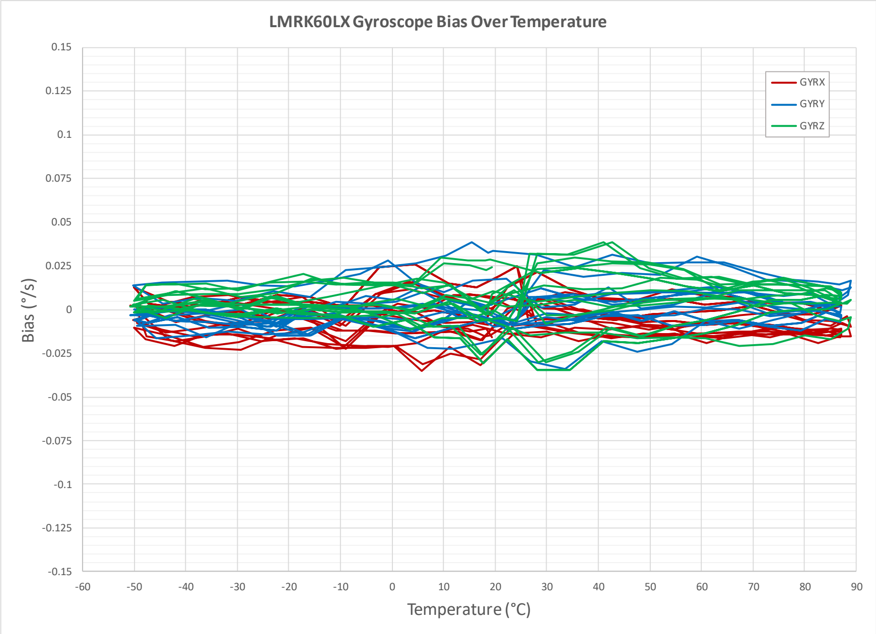
Raw gyroscope output bias over calibrated temperature range
