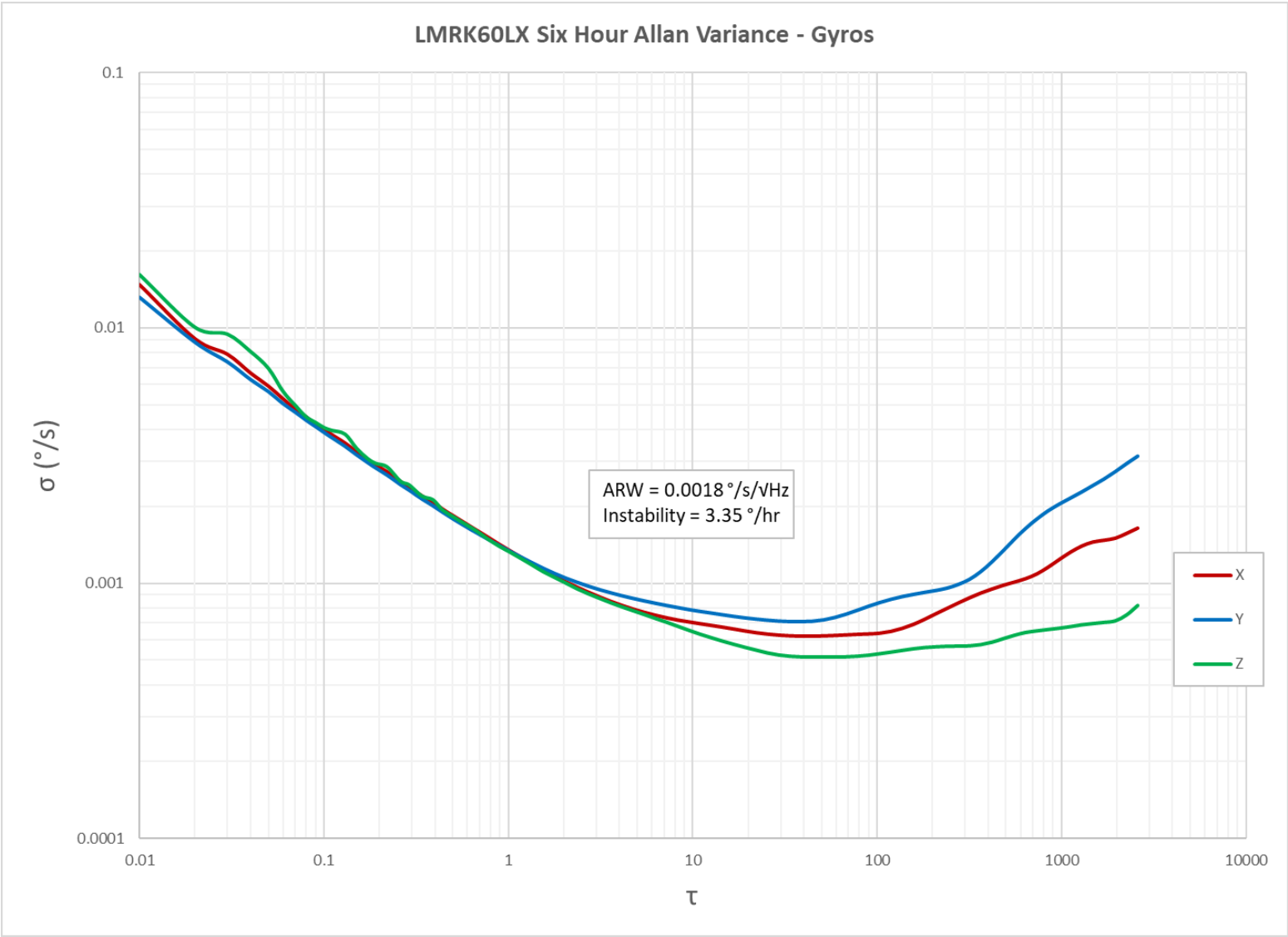
Gyroscope Allan-Variance (limited to 45 minutes)
