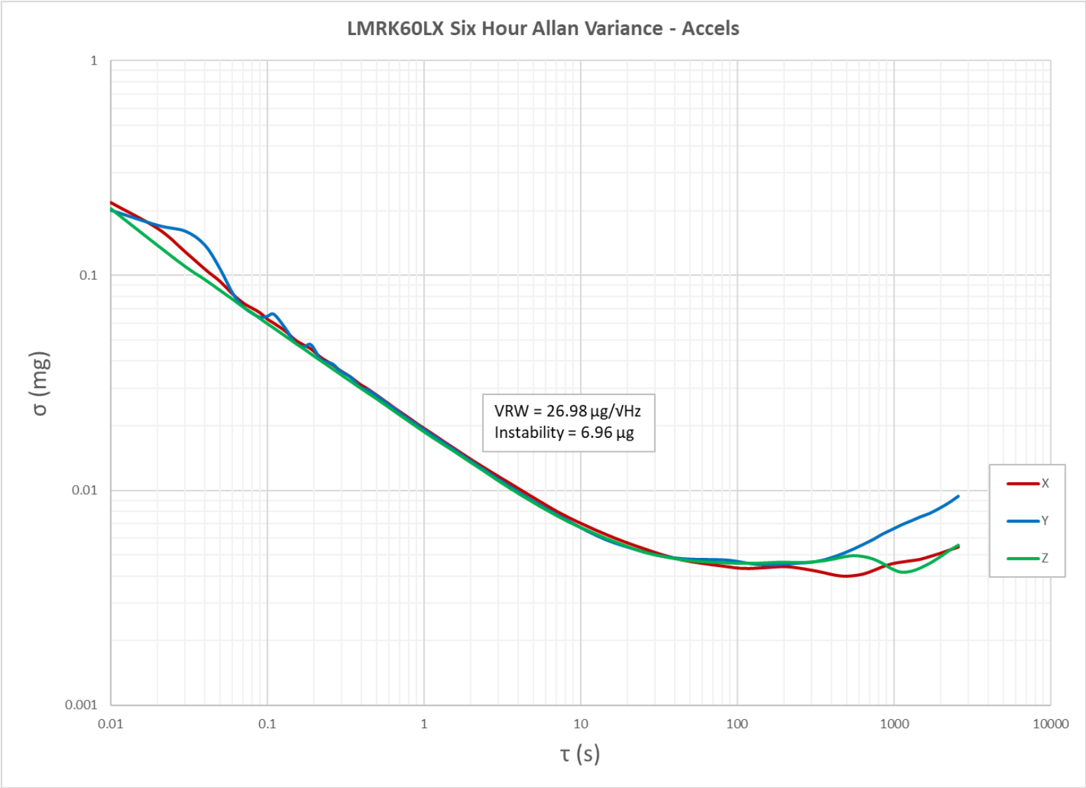
Accelerometer Allan-Variance (limited to 45 minutes)
