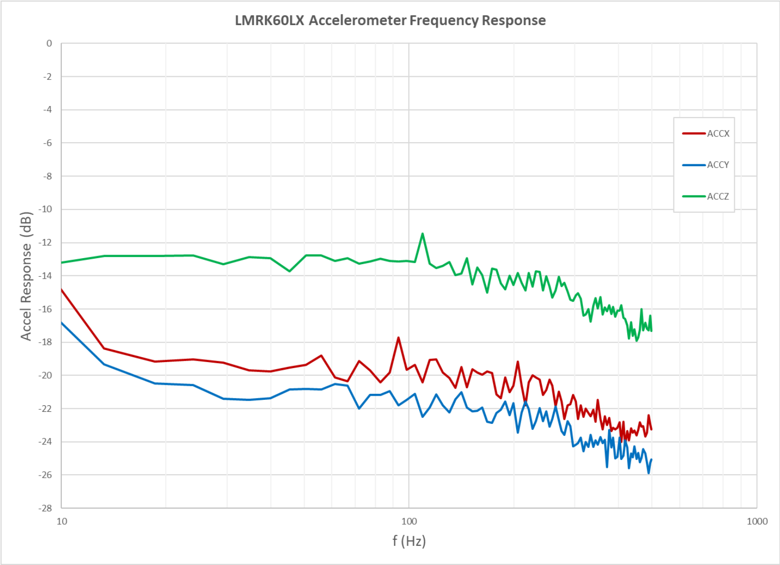
Accelerometer frequency response with LPF set to 250 Hz
