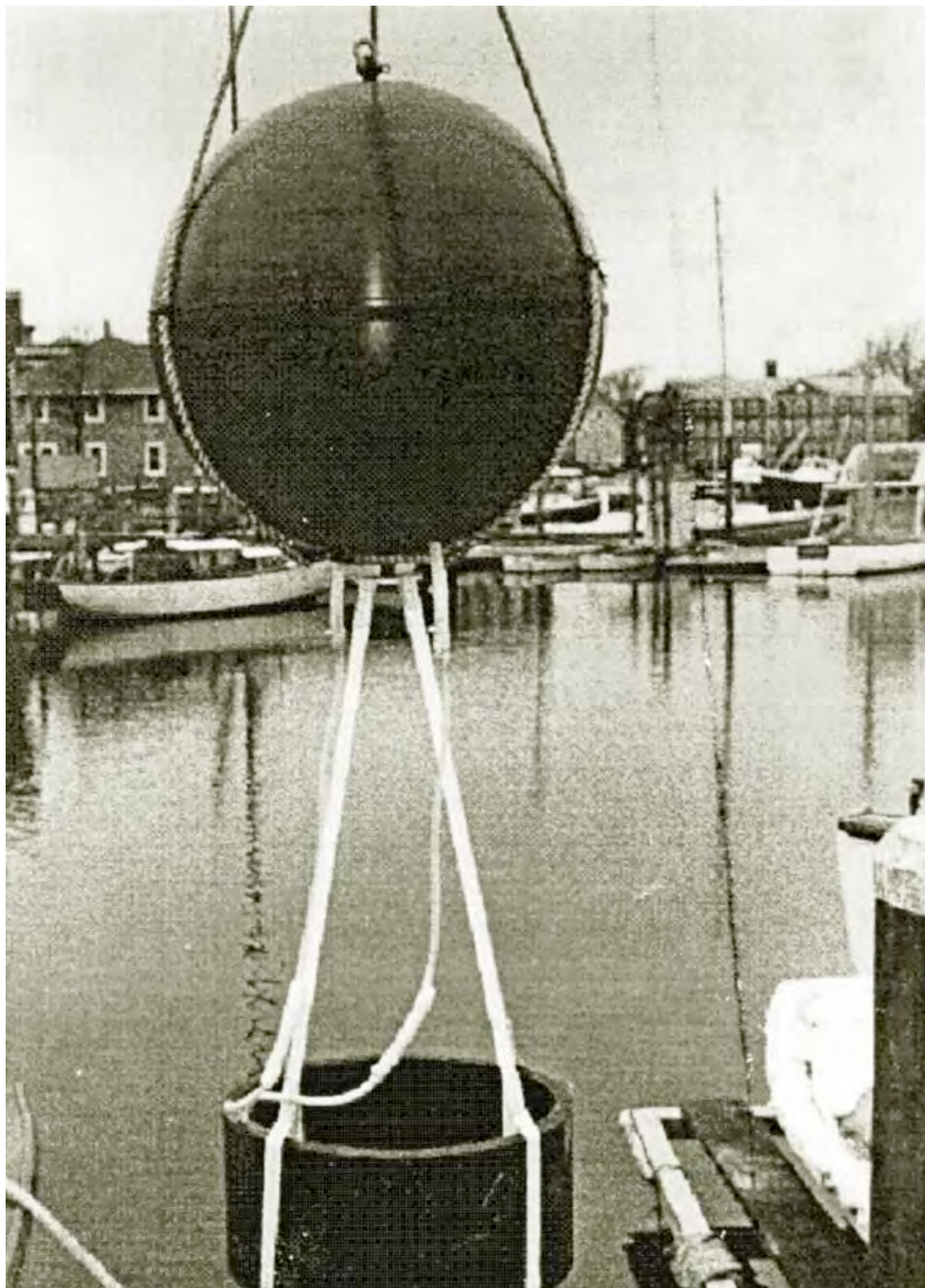
3) Prototype SOFAR float. (Photograph courtesy of Tom Rossby)
