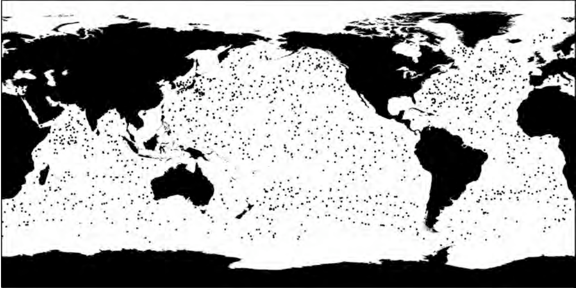
6) The global distribution of Argo floats in July 2004. (Argo Information Centre – http://www.argo.net ).
