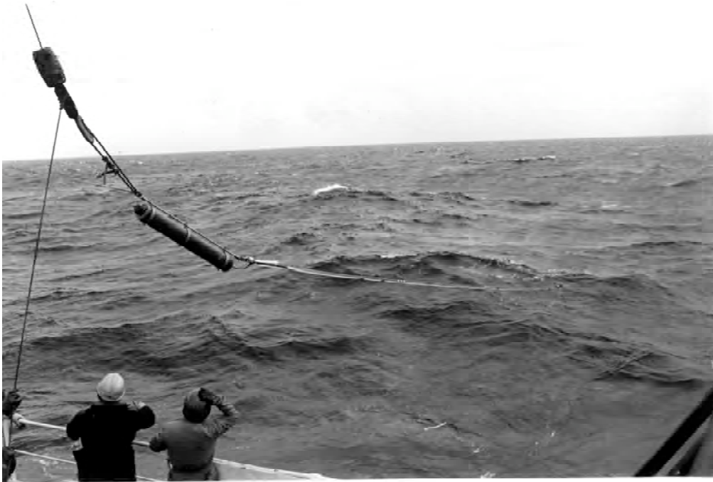
Figure 4 Recovery of an Autonomous Listening Station. Cylinder contains batteries and electronics, Outboard of the pressure case is the linear hydrophone array that is located below the electronics package. (Photograph, John Gould)
