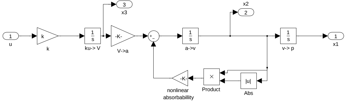
Figure 2.2: Simulink model of the dynamics of the robot
