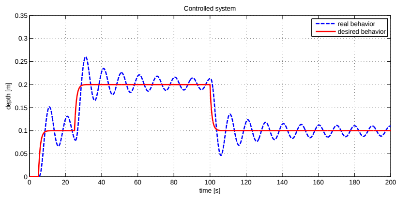
Figure 4.4: Behavior of the controlled PID system
