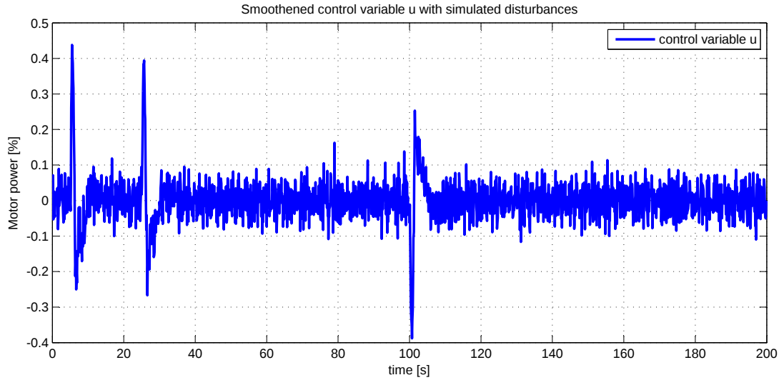
Figure 4.13: Control variable u with simulated disturbances smoothened by a PT1 term
