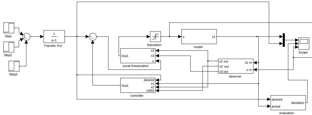
Figure 4.7: Complete Simulink plan with state feedback controller and exact linearization
