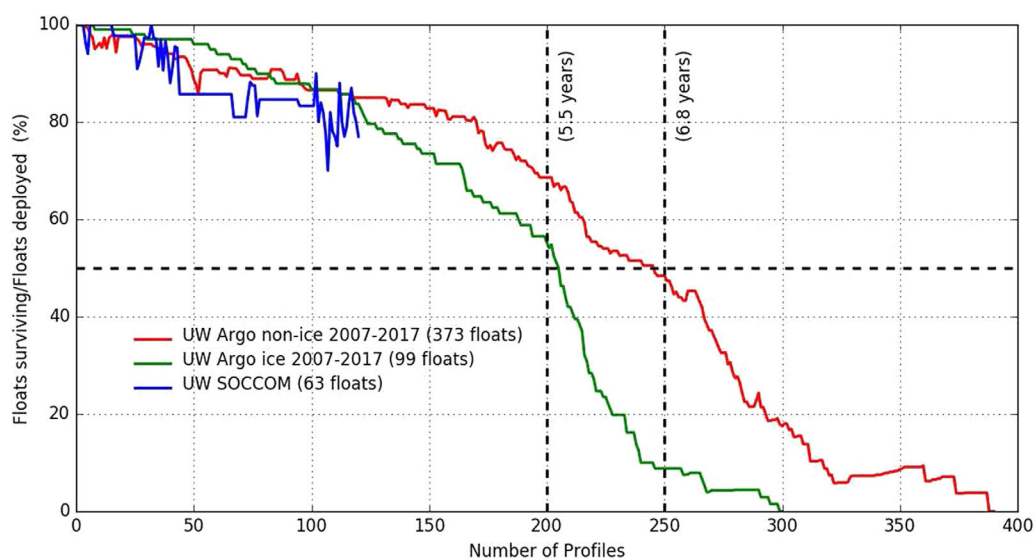
Figure 12. The total number of active floats compared to the number of floats deployed (%) as a function of number of profiles, for ensembles of non-ice Argo floats, Argo floats under sea ice, and SOCCOM floats. The horizontal dashed line denotes a value of 50% while the vertical dashed lines show times of 200 and 250 profiles (5.5 years and 6.8 years at 10-day cycling).
