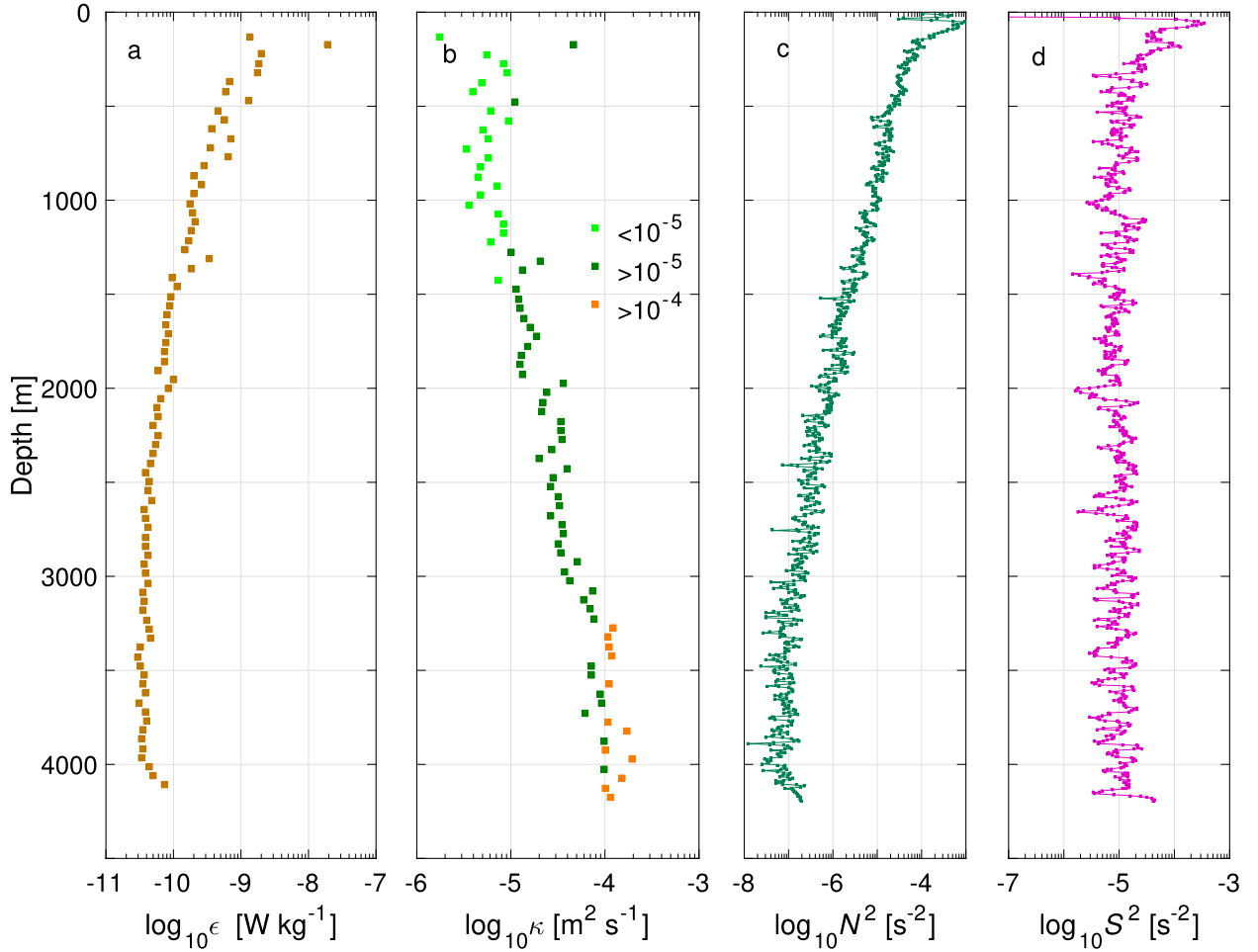
FIG. 12. Profiles of the rate of dissipation \varepsilon from (a) both probes, (b) the diapycnal eddy diffusivity \kappa , (c) the square of the buoyancy frequency N^2 , and (d) the square of the vertical shear S^2 , averaged into 50-m bins, for the sSCS.
