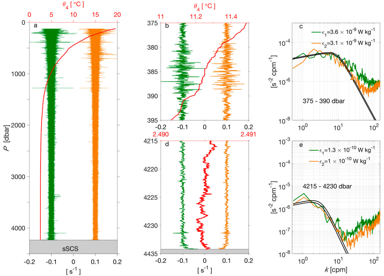
FIG. 7. Profiles of the microstructure shear from probe 1 (green, offset by -0.1 ) and probe 2 (gold, offset by 0.1 ), and the potential temperature relative to 4000 dbar (red) in the sSCS. (a) Full-depth view and (b), (d) selected depth ranges. The spectra of the shear for the pressure ranges (c) 375–390 and (e) 4215–4230 dbar. Triangles mark the limits of k_{\max} in (1). Thick lines are the Nasmyth spectra for the estimated rates of dissipation for each probe. Gray shading identifies the bottom.
