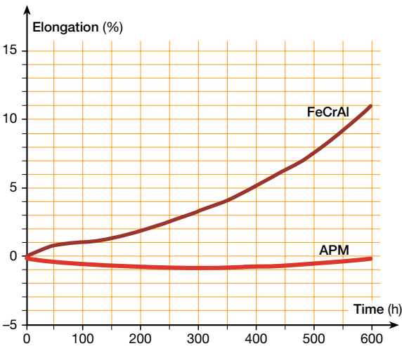
Fig. 1 Elongation at 2370°F element temperature.
