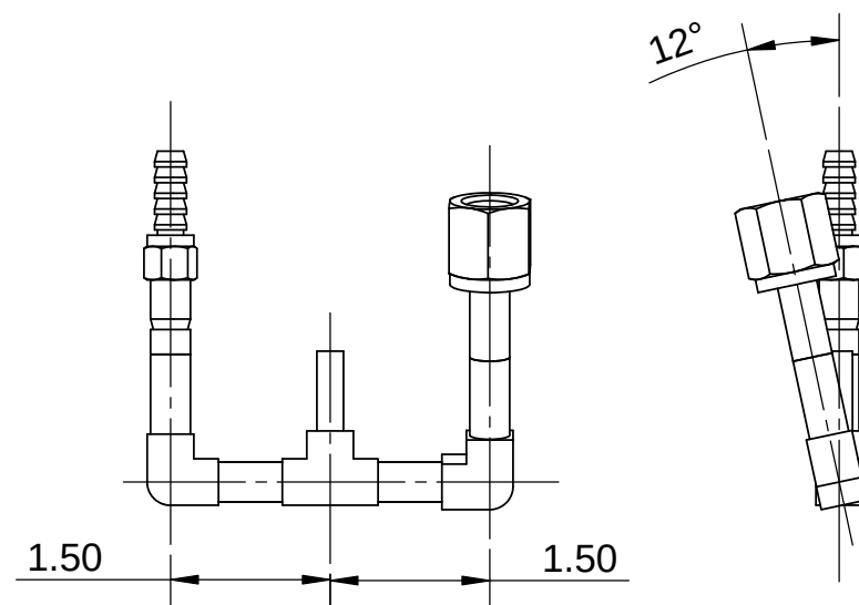
Reservoir Side
