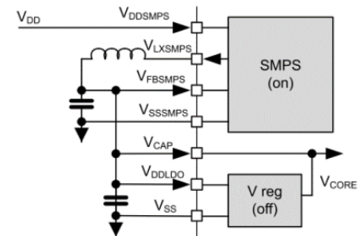
Figure 12. Config2 - SMPS only (Default configuration)
