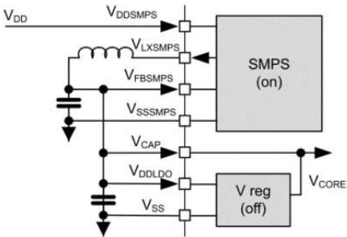
Figure 12. Config2 - SMPS only (Default configuration)
