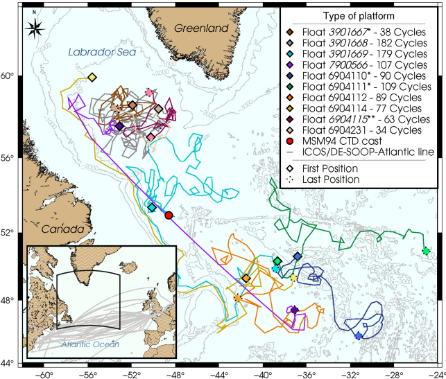
Figure 1. Map of the northwest Atlantic with the Labrador Sea and North Atlantic Current showing the trajectories of all 10 pH / O 2 floats deployed so far in our pilot study. In the legend, floats in italics are inactive. * Float with a faulty pressure and/or pH sensor. ** Float recovered. Dotted points show the last locations as of 7 February 2023. In the inserted map, gray lines indicate the corridor and discrete ship routes occupied by our ship-of-opportunity platform (ICOS station DE-SOOP-Atlantic Sail) during the period 2021–2022. The red dot indicates the location of hydrographic station 13 visited during the Maria S. Merian cruise 94 (MSM94) in August 2020.
