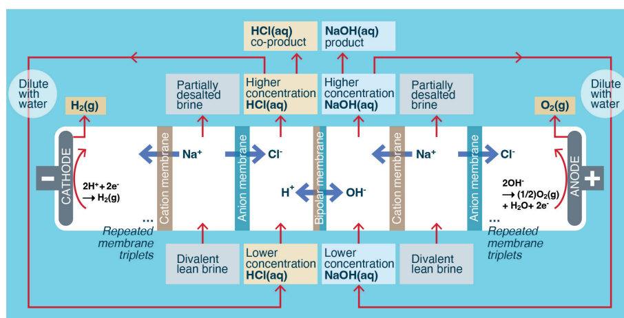
Figure 5. Typical process flow for the electrodialytic conversion of aqueous brine into alkalinity.
