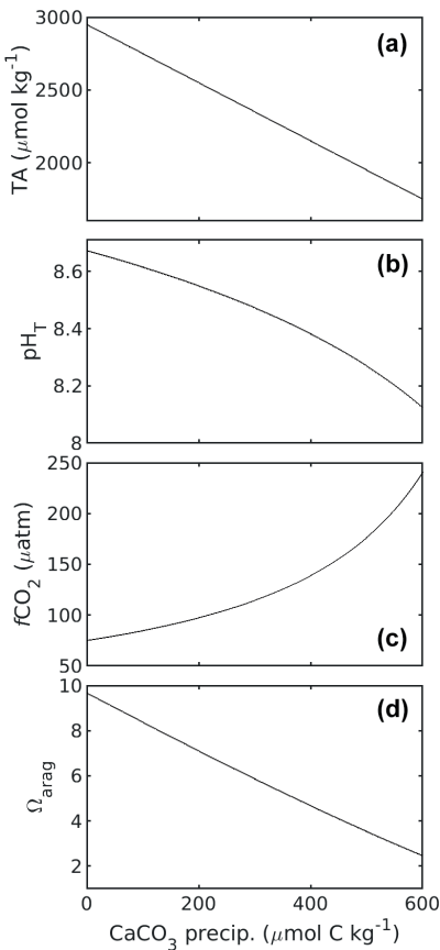
Figure 3. Changes in TA (a), pH T (b), f CO 2 (c), and Ω arag (d) in response to CaCO 3 precipitation, i.e. DIC removal. Carbonate chemistry calculations for a salinity of 35 at 20 °C were as described in the caption of Fig. 1. Starting TA and DIC were 2950 and 2100 μmol kg –1 . Please note that for 1 mol of CaCO 3 precipitated, 1 mol of DIC is consumed.
