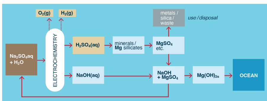
Figure 7. Example of the indirect production of solid, polyvalent metal hydroxides from minerals and water using electrochemistry or electrolysis of a monovalent salt. \text{H}_2 and \text{O}_2 are also produced.
