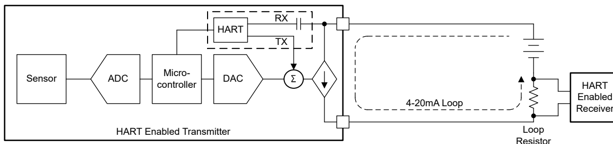
Figure 1-2. Adding HART to the 4-20 mA Loop
