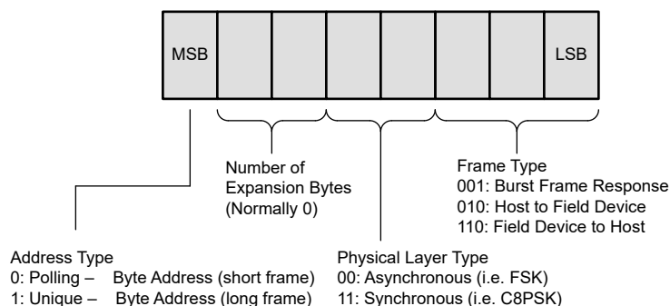
Figure 1-10. HART Start Byte
