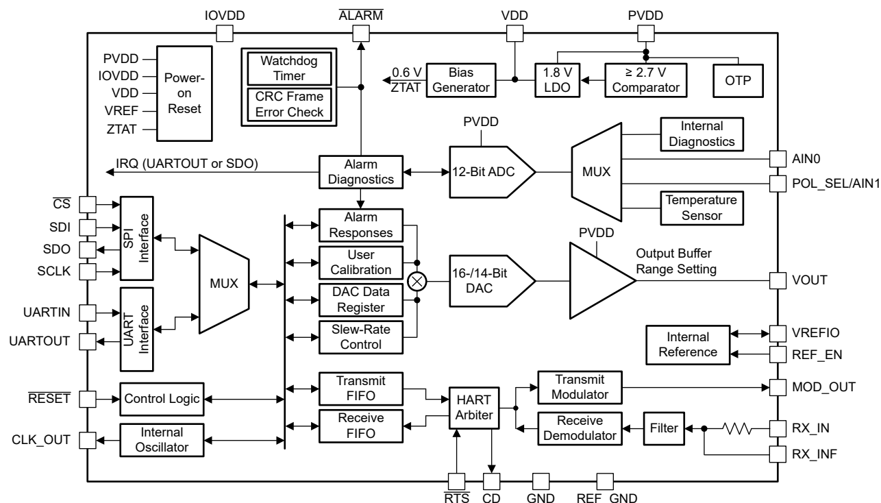
Figure 3-5. Block Diagram of the AFEx81H1 and AFEx82H1 HART Modem
