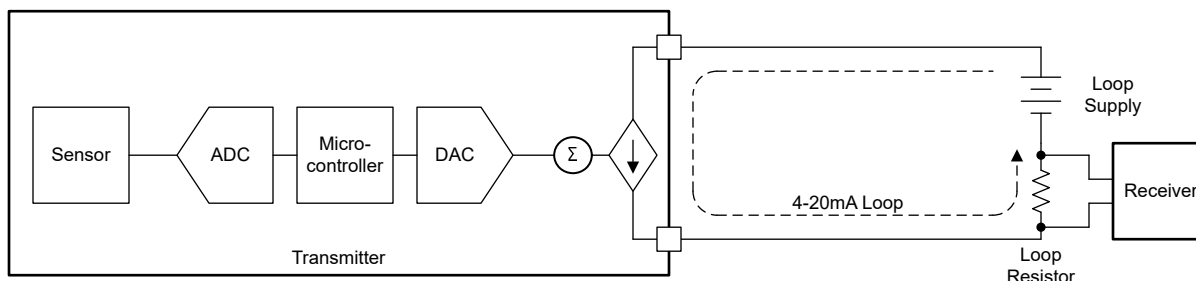
Figure 1-1. A Remote Transmitter on a 4-20 mA Loop
