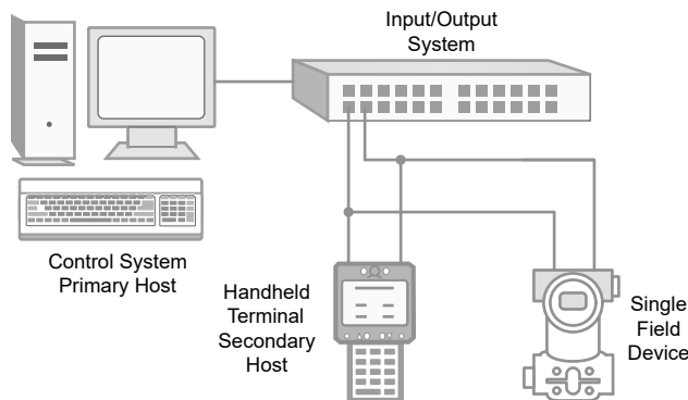
Figure 1-5. Point-to-Point Connection for a HART Host and a HART-Enabled Field Transmitter
