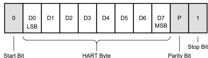
Figure 1-9. The HART Protocol Byte
