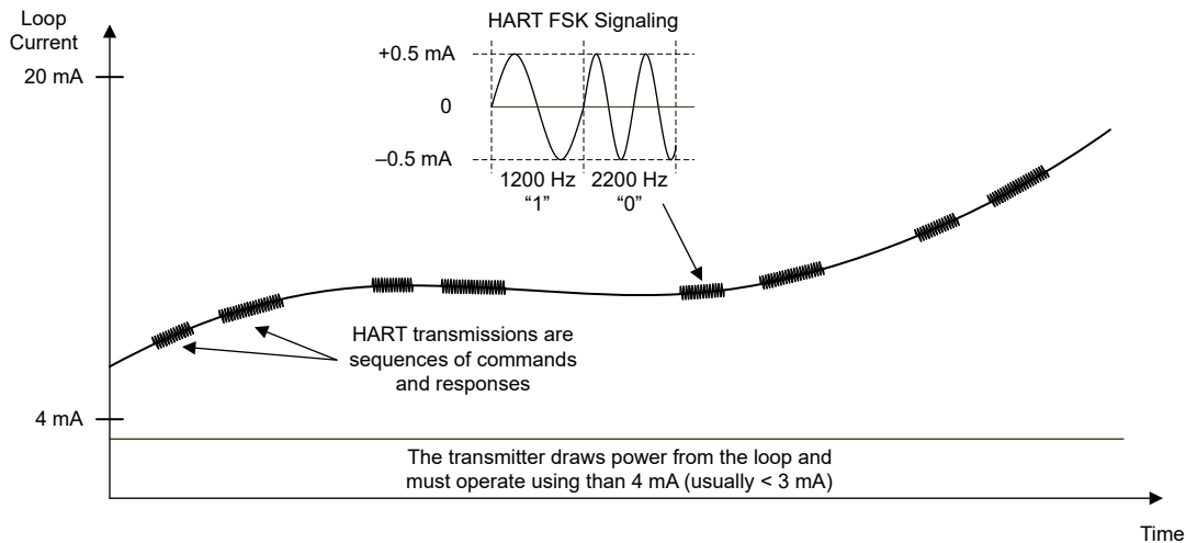
Figure 1-3. HART Transmissions on a 4-20 mA Loop
