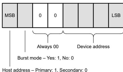
Figure 1-11. HART Short Frame Address Byte
