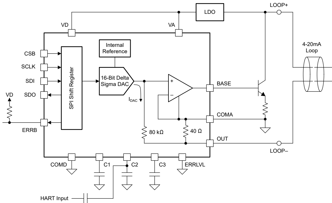
Figure 3-1. Block Diagram of the DAC161S997 in a Field Transmitter Application
