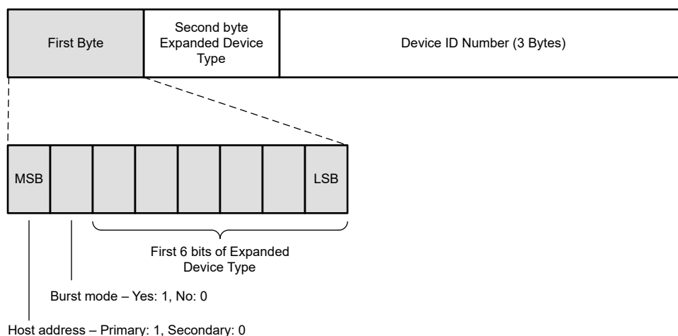
Figure 1-12. HART Long Frame Address
