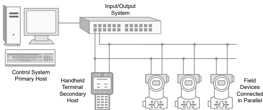
Figure 1-6. Field Transmitters Set Up in HART Multi-Drop Mode
