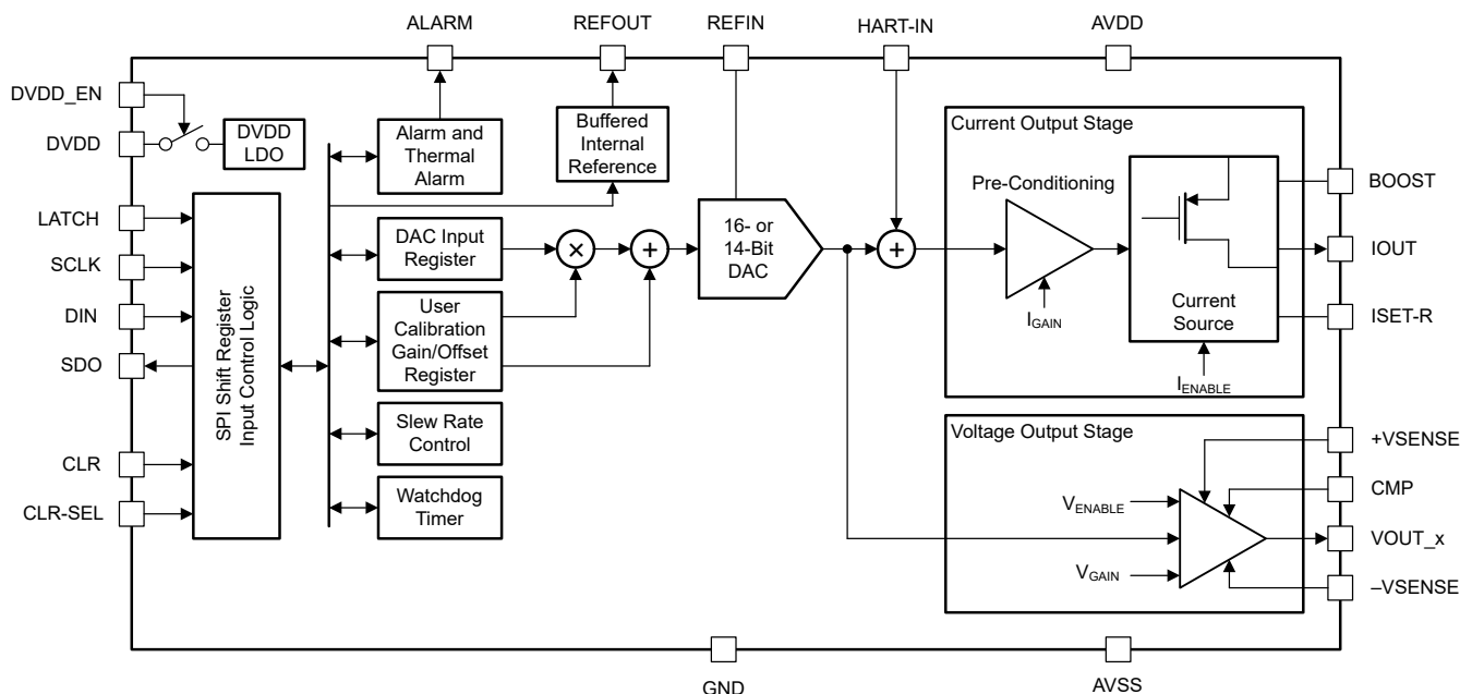
Figure 3-2. Block Diagram of the DAC8760
