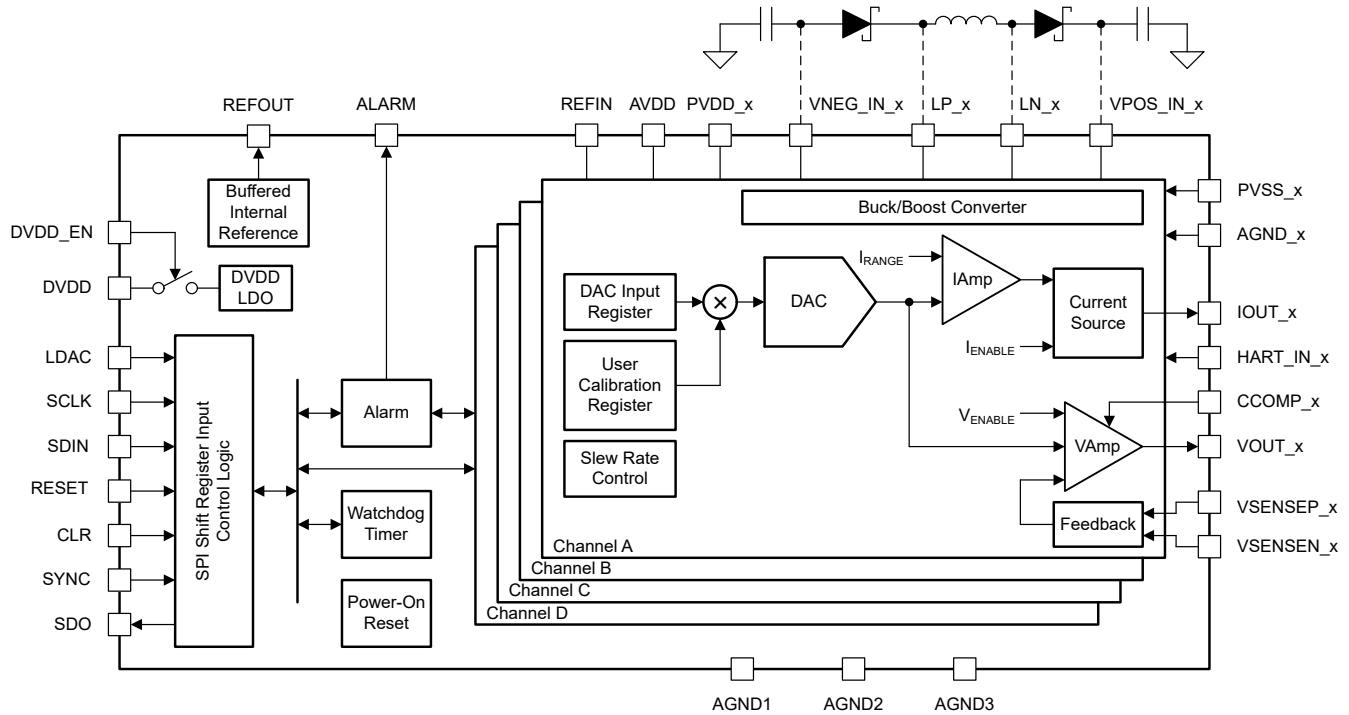
Figure 3-3. Block Diagram of the DAC8775
