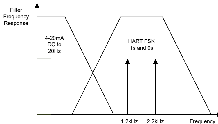
Figure 1-4. Filtering for the Primary Variable and HART FSK
