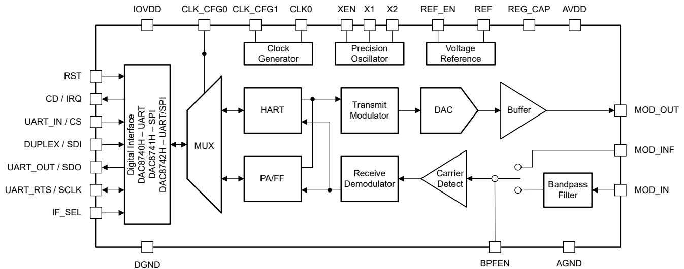
Figure 3-4. Block Diagram of the DAC874xH HART Modem
