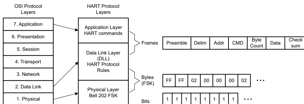
Figure 2-1. HART Protocol Compared to the OSI Protocol Model
