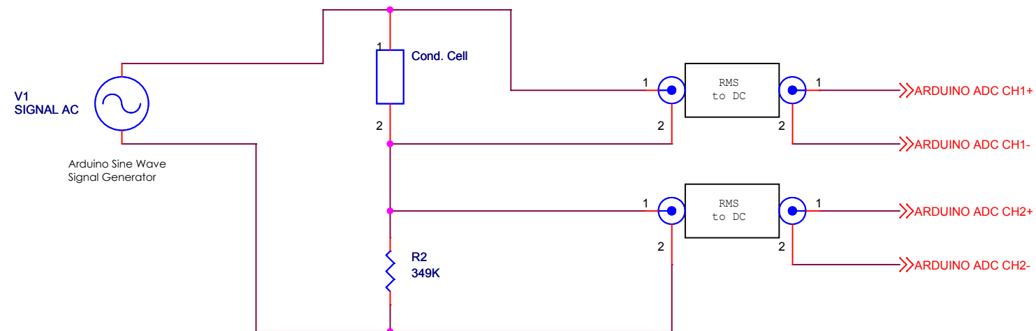
Conductivity Cell Schematic (Arduino)
