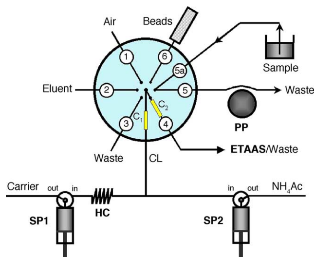
Fig. 1. SI-LOV system for determination of ultra-trace levels of Cd, Pb and Ni using preconcentration by chelating Sepharose beads and detection by ETAAS. SP1 and SP2, syringe pumps; PP, peristaltic pump; CL, communication line; C 1 and C 2 , microcolumn positions (although these for clarity are shown wider, all channels in the LOV are actually of identical internal diameter (1.66 mm)).
