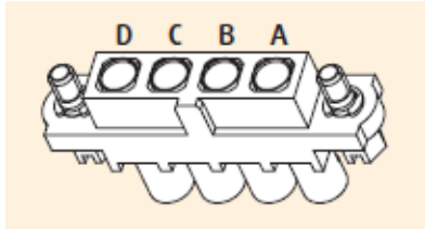
Harwin Datamate Mix-Tek Numbering
