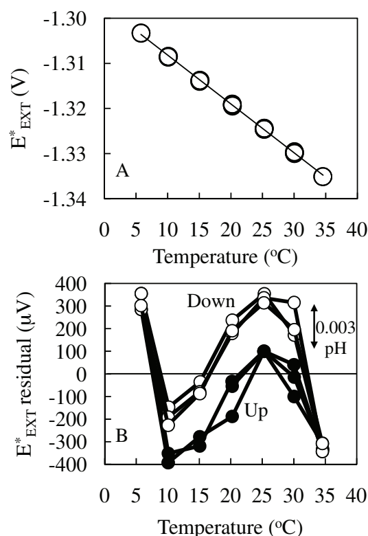
Fig. 4. (A) Standard potential of a FET|EXT calculated using Eq. 10; same data used to calculate \partial E_{\text{EXT}}^*/\partial T for TRIS in Table 1. (B) Residuals from the linear fit shown in panel A. Sensors were operated using a Cap Adapter and voltages were recorded using a National Instruments 9219.
