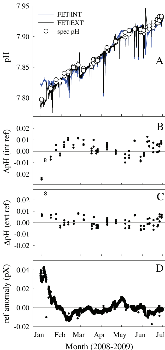
Fig. 5. (A) Six months of continuous operation in the MBARI test tank for a single Durafet using both the internal reference electrode and an external CI-ISE. Discrete samples were collected by bottle and measured using standard spectrophotometric pH protocols. (B) and (C) show residuals between the sensor and discrete measurements for the internal and external reference electrodes, respectively. (D) The difference between the two reference half cells, attributed mostly to drift in the liquid junction potential. Sensors were operated using a Cap Adapter and voltages were recorded using a National Instruments 9219.
