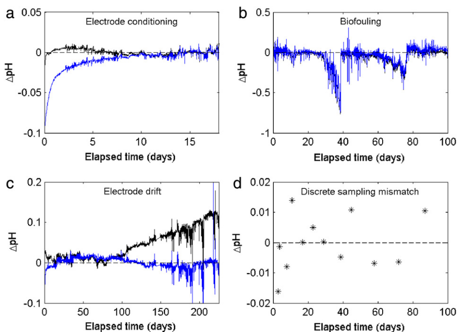
Fig. 5. Composite of anomaly time-series from (a) Scripps Test Tank SeapHOx, (b) L20 Mooring SeaFET2, (c) Del Mar Buoy SeaFET, and (d) L20 Mooring SeapHOx. Black and blue represent \Delta\text{pH}^{\text{INT-ref}} and \Delta\text{pH}^{\text{EXT-ref}} , respectively. Reference pH values are (a) spectrophotometric, (b) \text{pH}^{\text{INT}} from a stable SeapHOx, (c) \text{pH}_{\text{O}_2}^{\text{EST}} , and (d) discrete sample values. Black dashed lines represent a zero anomaly. Note that y-axis limits differ among the four deployments, indicating that there can be significant differences in the magnitudes of various errors. (For interpretation of the references to color in this figure legend, the reader is referred to the web version of this article.)
