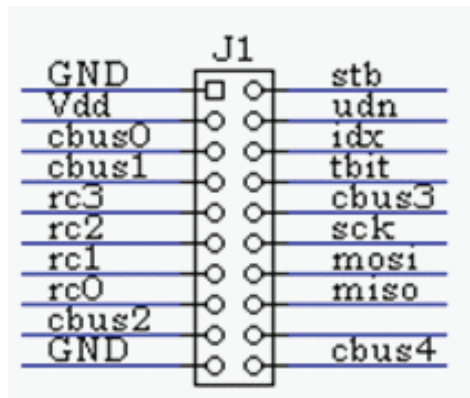
Figure 10: Expansion connector
