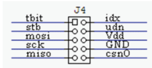
Figure 9: Encoder connector
