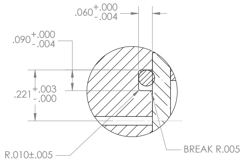
DETAIL A SCALE 4 : 1
