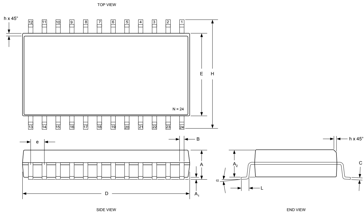
Figure 14-2: Package Outline Drawing SOP24, 300 MILS
