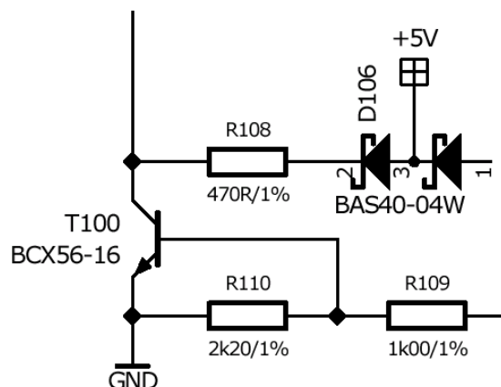
Figure 3.5 Outputs (OUT 0 , OUT 1 )
