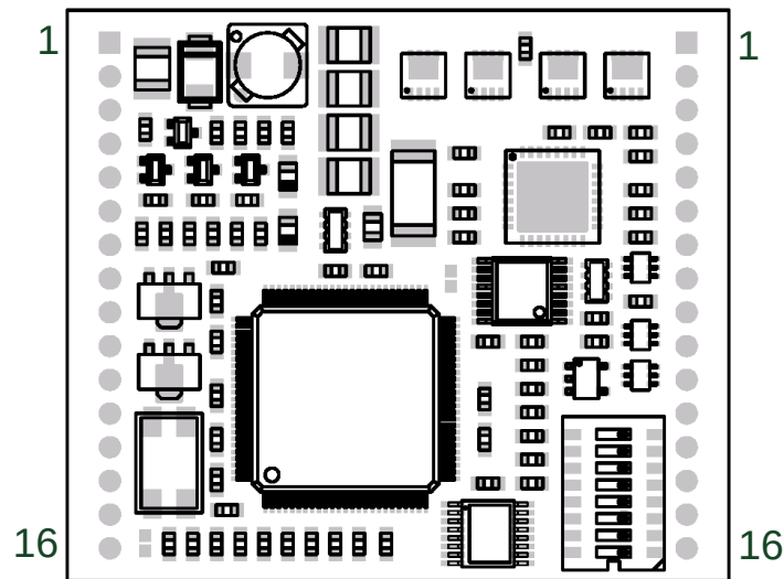
Figure 3.2 TCM-103 connectors
