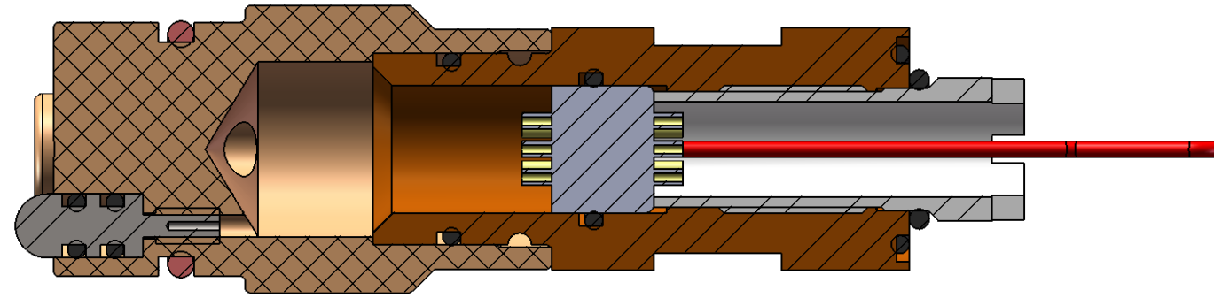
SECTION H-H SCALE 3 : 2
