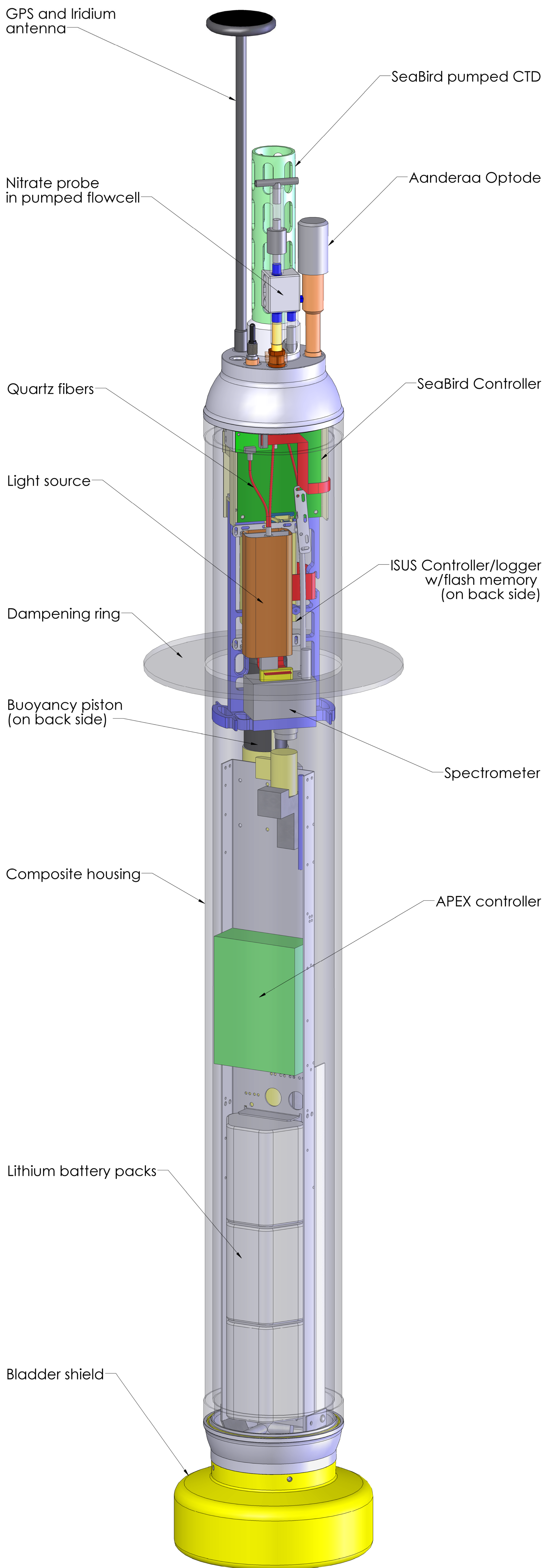
The APEX+ISUS Float Version 2 Jannasch/MBARI, Sept 2008, Scale 1:2
