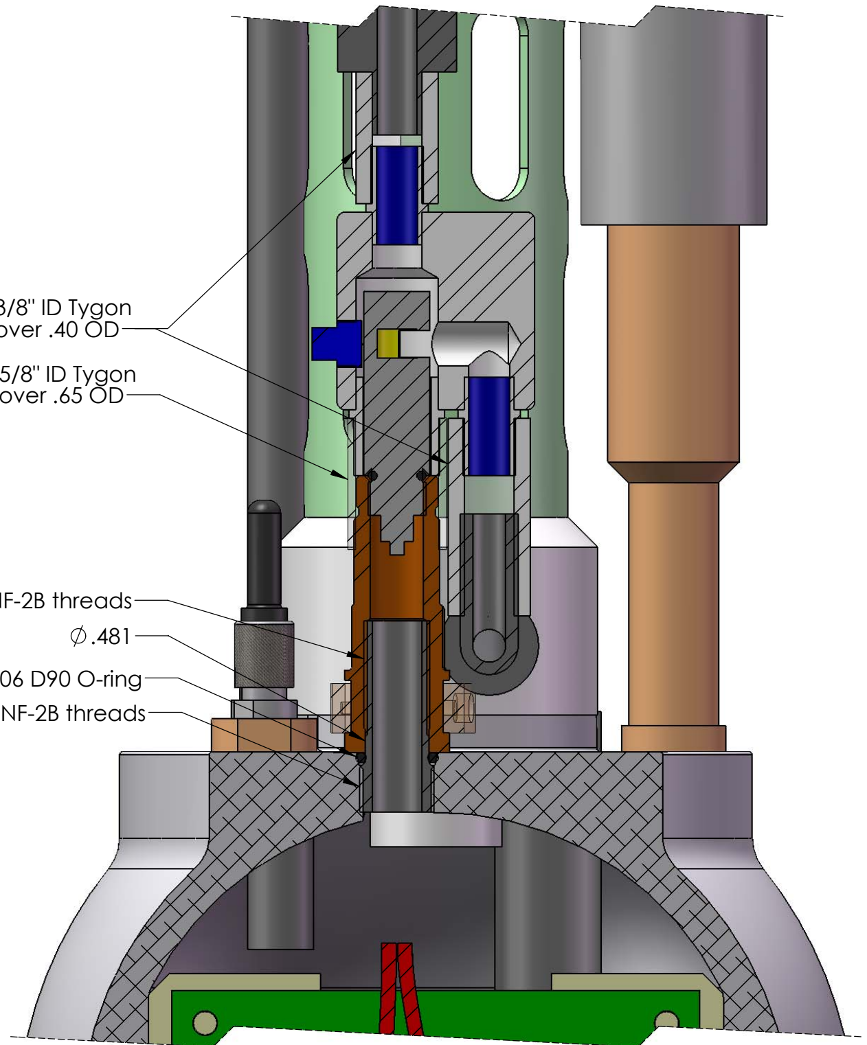
APEX+ISUS Ver2 EquiTech probe fitting per Positionable SAE#6 fitting
