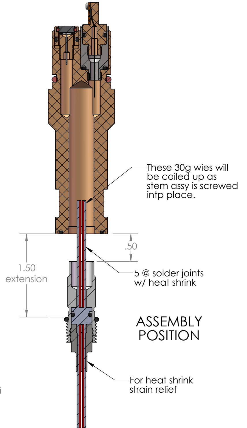
SECTION C-C SCALE 1 : 1
