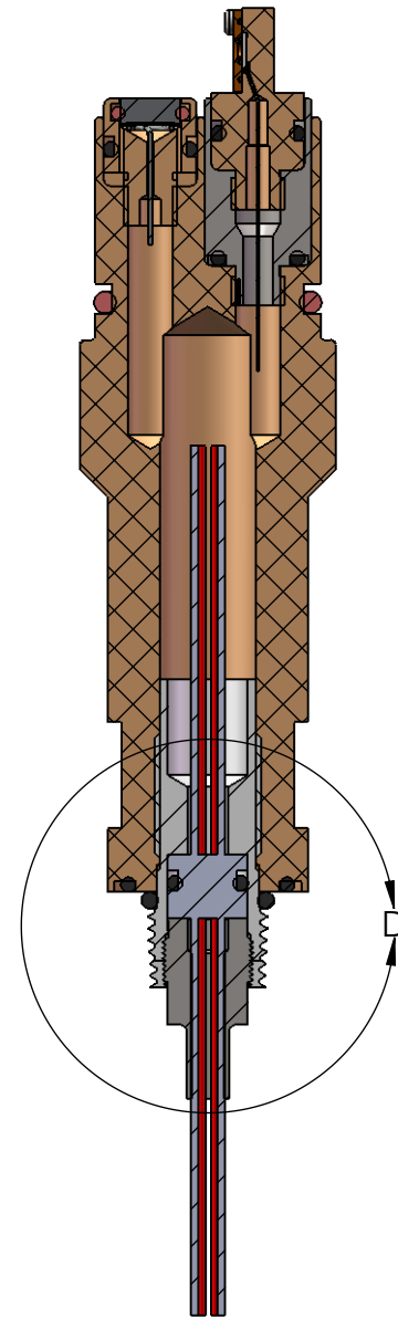
SECTION C-C SCALE 1 : 1
