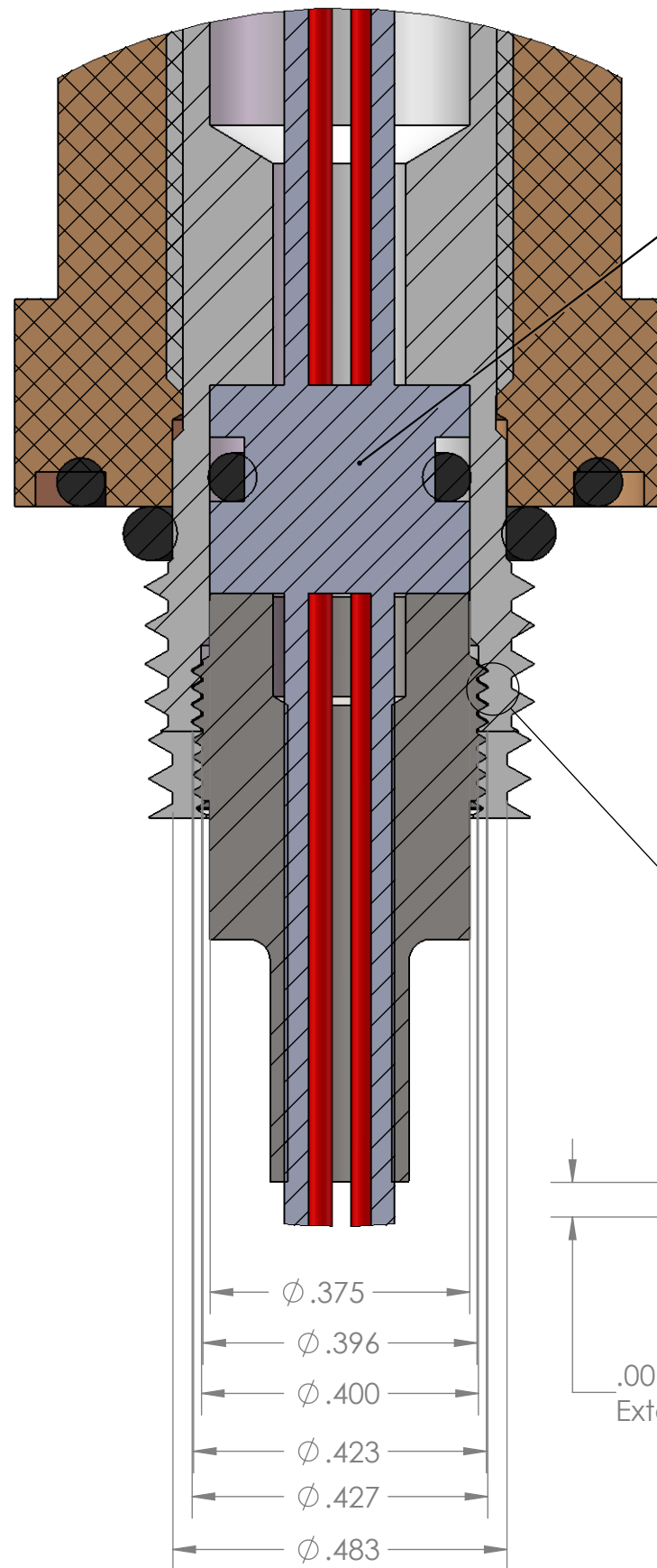
DETAIL D SCALE 4 : 1
