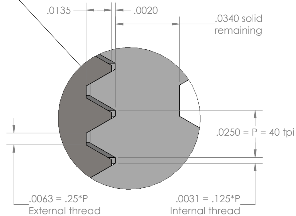
DETAIL E SCALE 32 : 1
