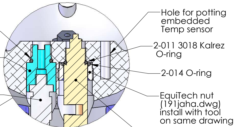
DETAIL B SCALE 1 : 1
