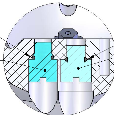
DETAIL C SCALE 1:1 Plugged for pressure testing
