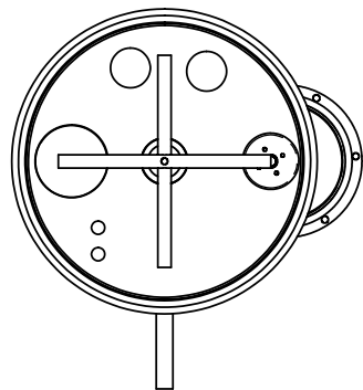
Benthic Chamber Concept Hans Jannasch/MBARI Version 2; 3/21/07
