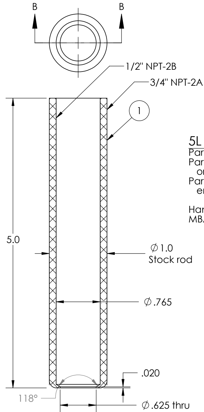
SECTION B-B SCALE 1 : 1
