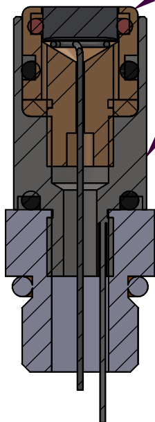
SECTION C-C SCALE 2 : 1
