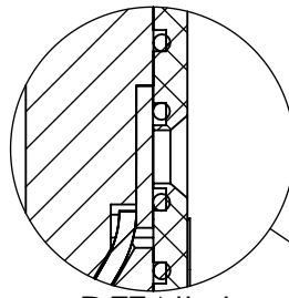
DETAIL J SCALE 4 : 1
