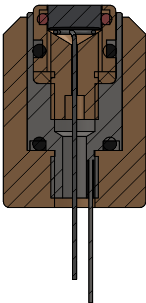
SECTION G-G
