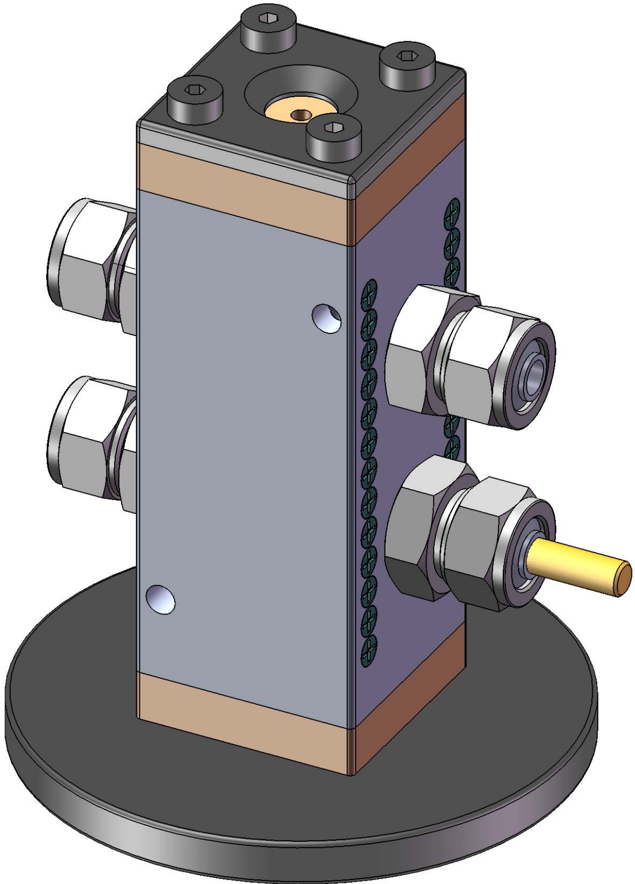
Pressure/Temperature Cell Concept HWJ/MBARI 3/20/09
