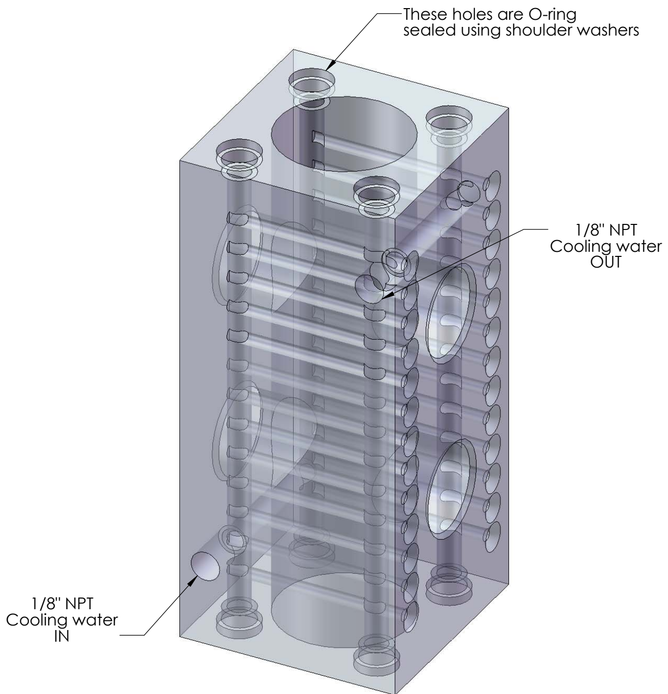
Pressure/Temperature Cell Concept HWJ/MBARI 3/20/09
