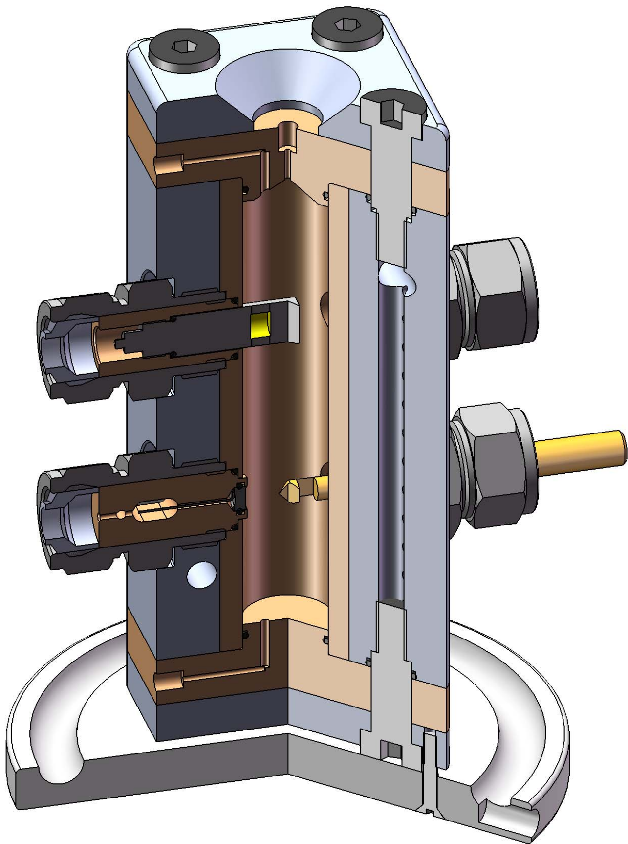
Pressure/Temperature Cell Concept HWJ/MBARI 4/20/09
