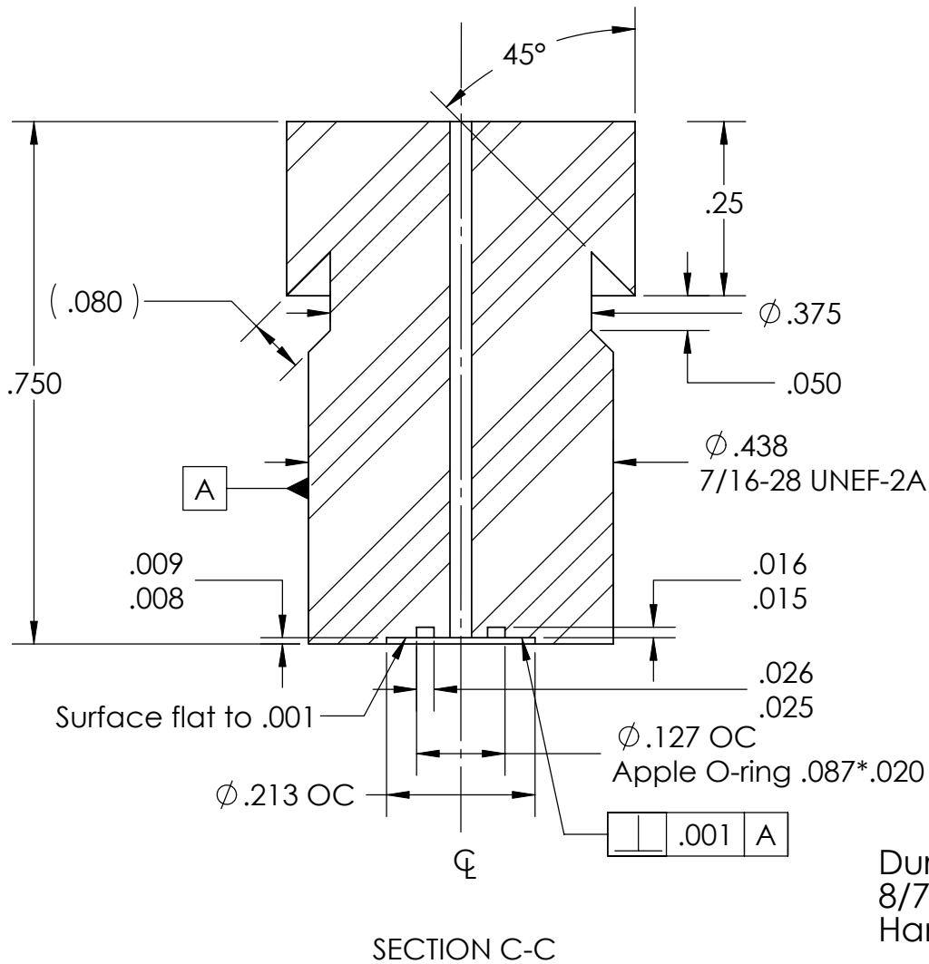
Chip retainer Qty: 2 Material: PEEK
