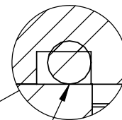
DETAIL B SCALE 16 : 1
