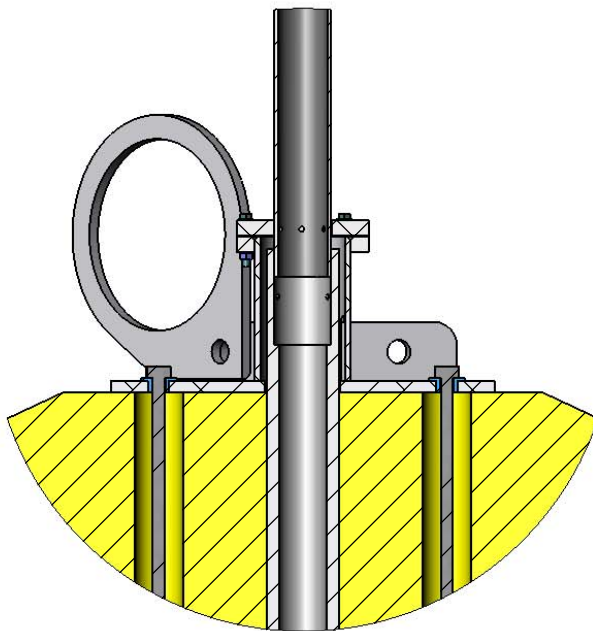
DETAIL C SCALE 1 : 8
