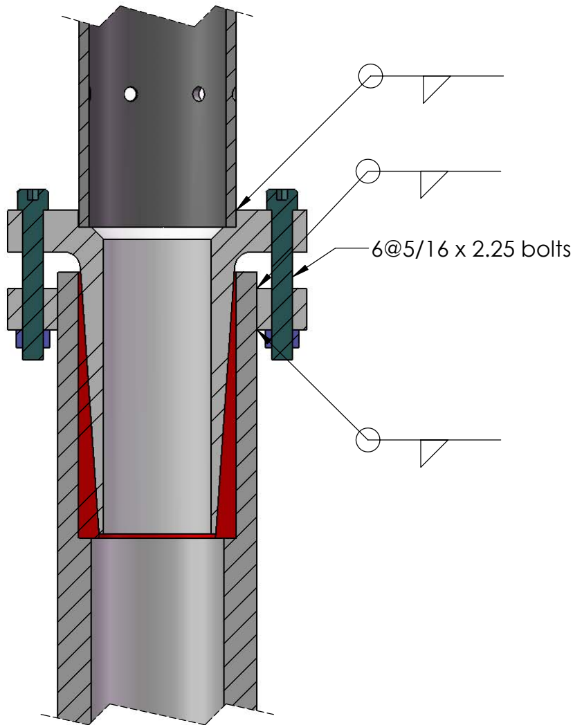
DETAIL A SCALE 1 : 4
