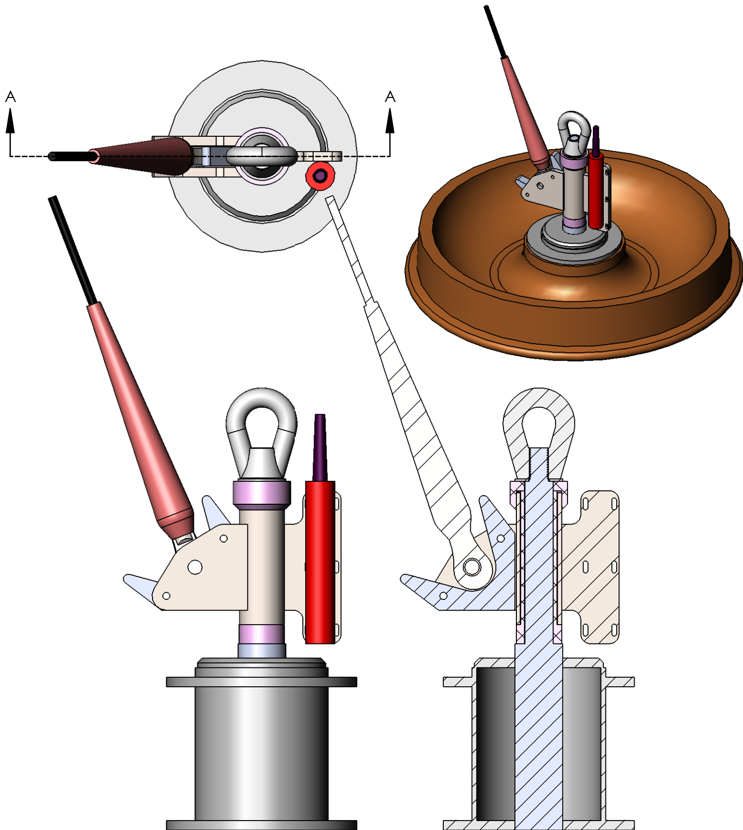
LOBO Swivel Anchor for line with flotation Hans Jannasch/MBARI Concept 1/9/14
