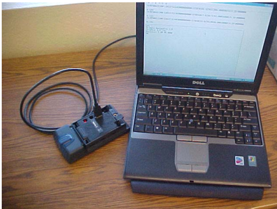
Figure 33. TrimTrac Pro Connected to PC via Provisioning Module and USB A-to-A Cable.
