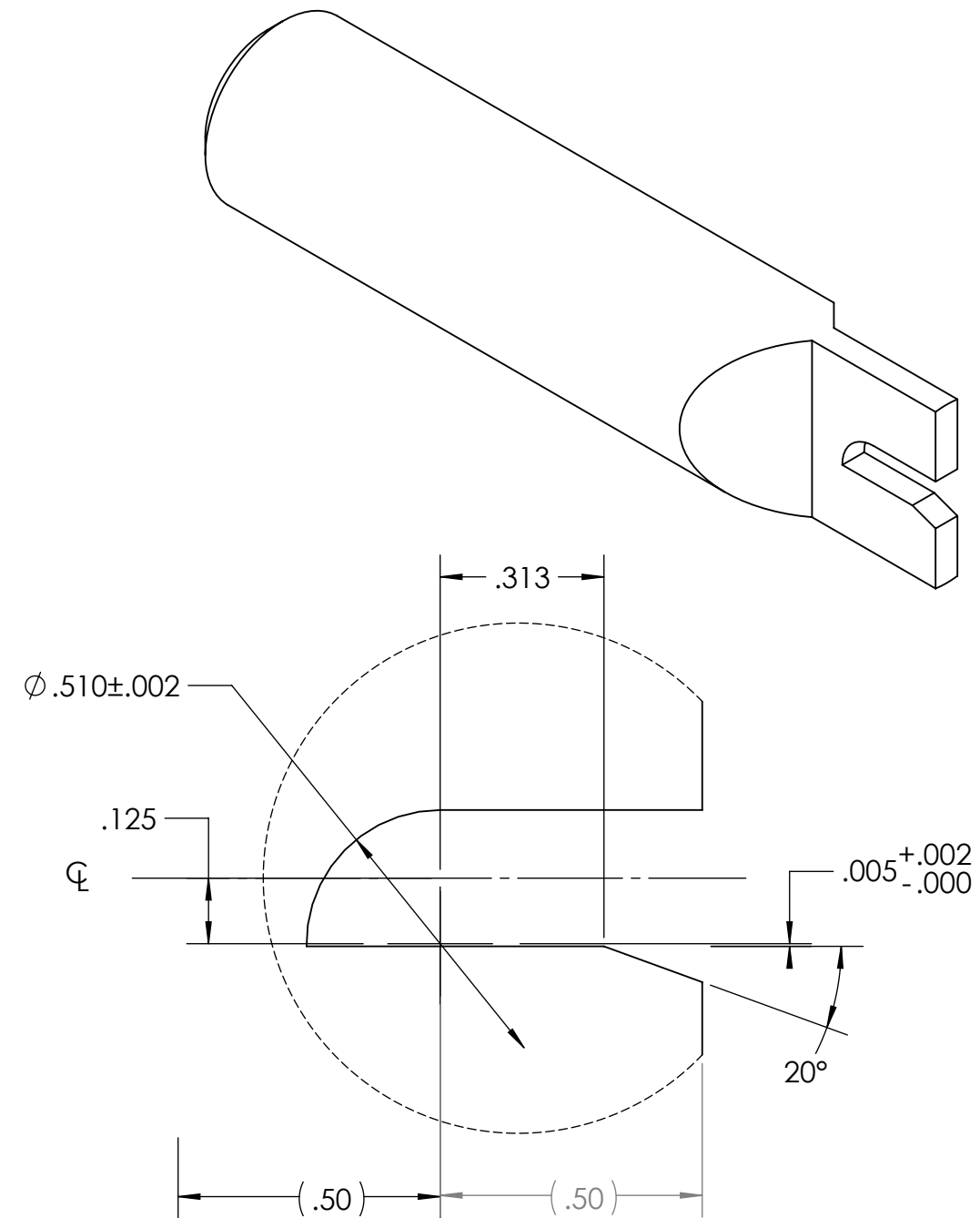
DETAIL A SCALE 3 : 1
