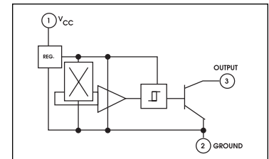
Sinking Block Diagram
