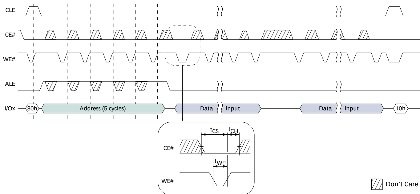
Figure 68: Program Operation with CE# “Don’t Care”
