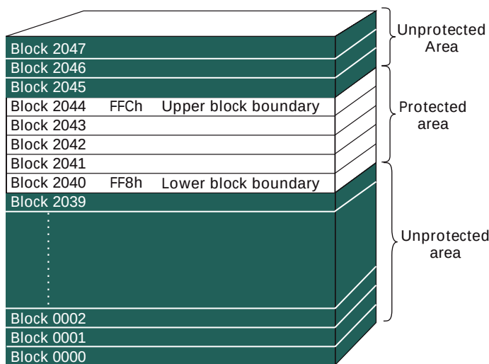
Figure 32: Flash Array Protected: Invert Area Bit = 1
