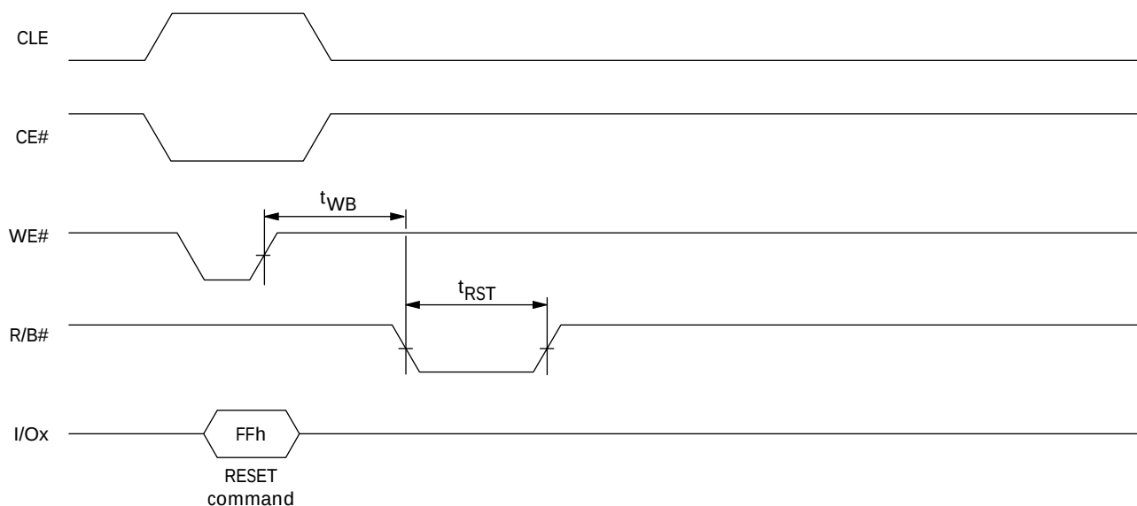
Figure 46: RESET Operation
