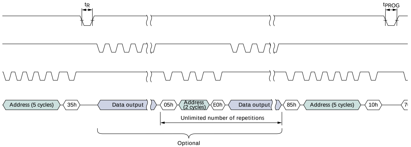
Figure 28: INTERNAL DATA MOVE
