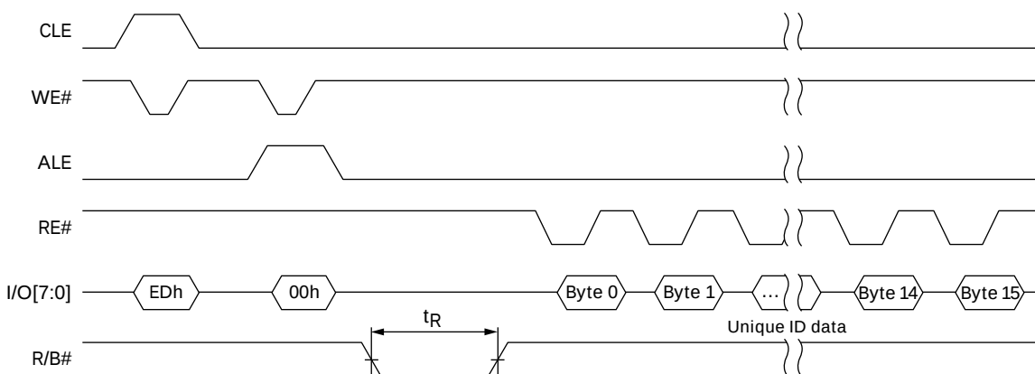
Figure 22: READ UNIQUE ID Operation
