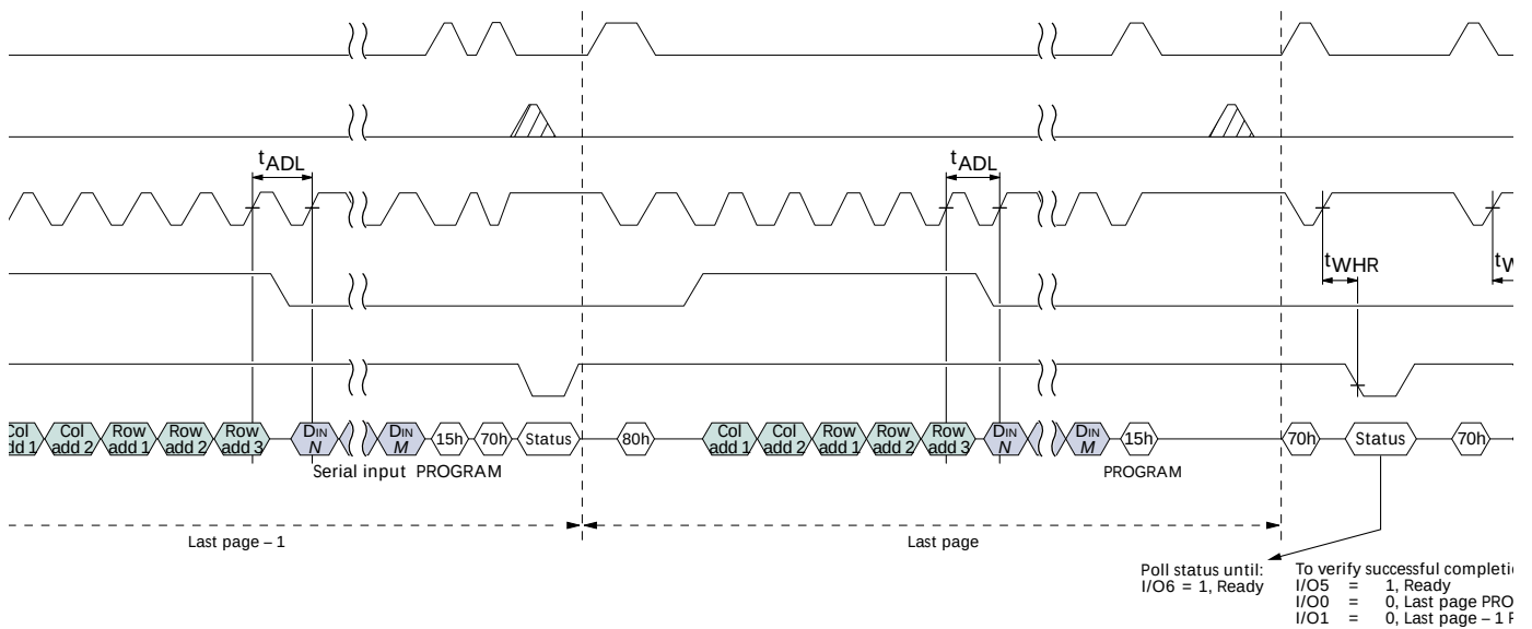
Figure 72: PROGRAM PAGE CACHE MODE Operation Ending on 15h
