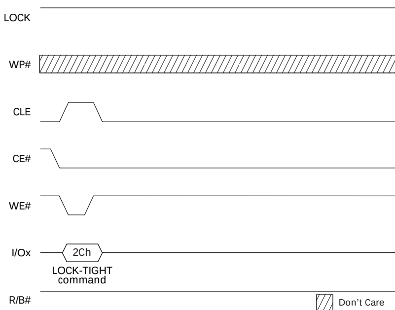
Figure 35: LOCK-TIGHT Operation
