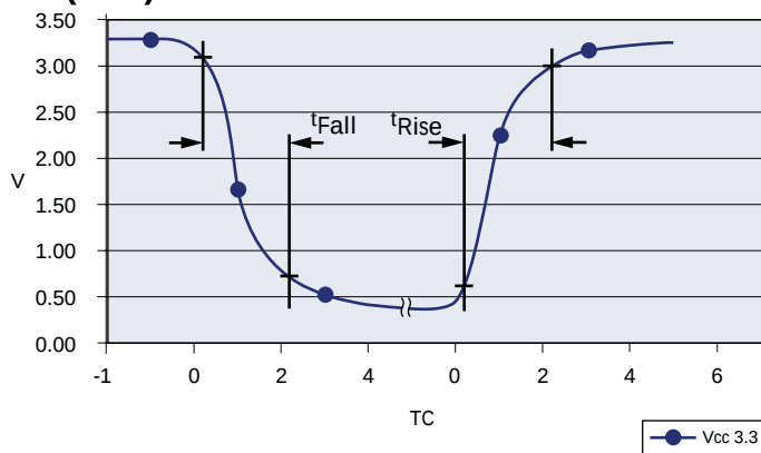
Figure 13: t_{\text{Fall}} and t_{\text{Rise}} (3.3V)
