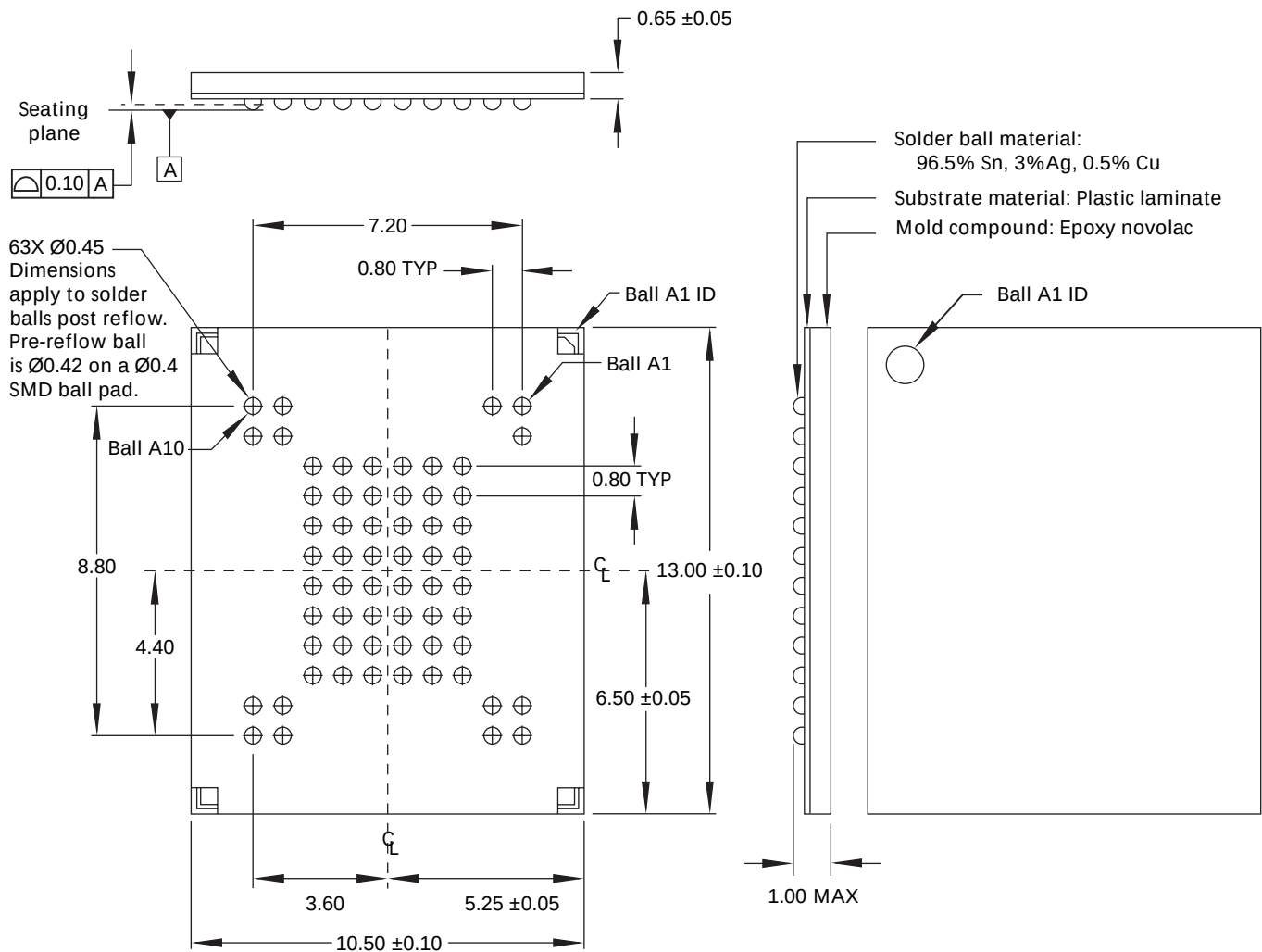
Figure 76: 63-Ball VFBGA
