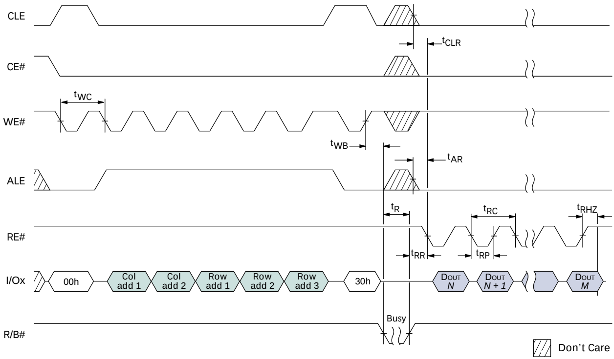
Figure 59: PAGE READ Operation
