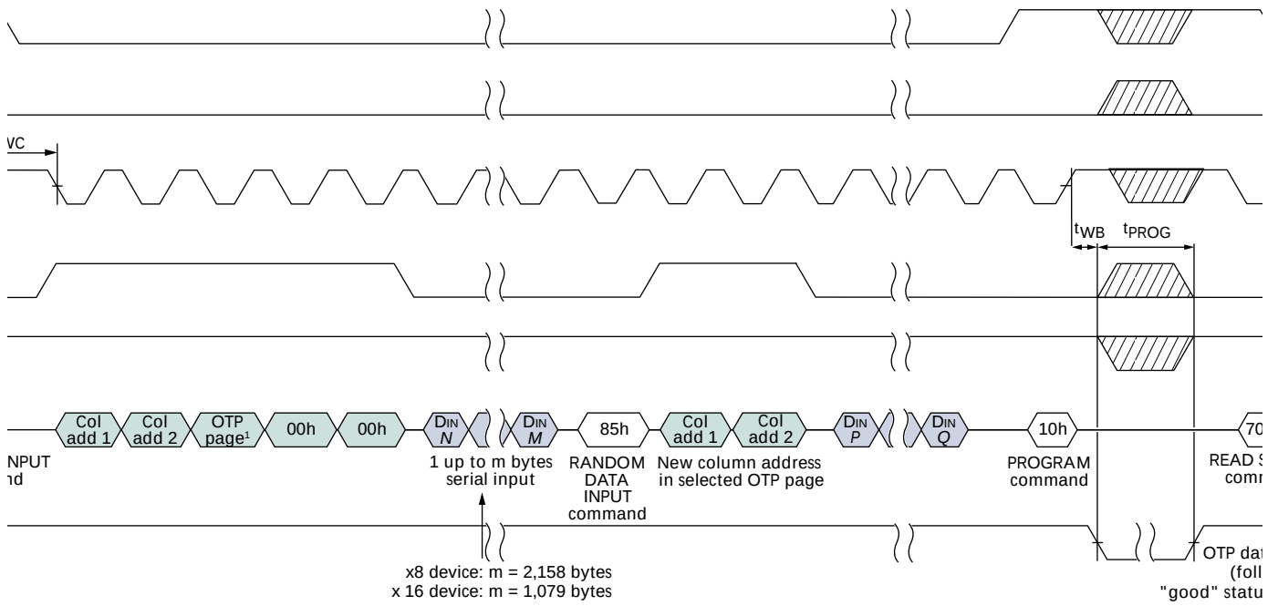
Figure 40: OTP PROGRAM with RANDOM DATA INPUT
