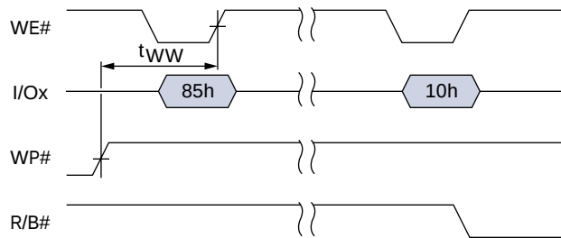
Figure 51: PROGRAM for INTERNAL DATA MOVE Enable
