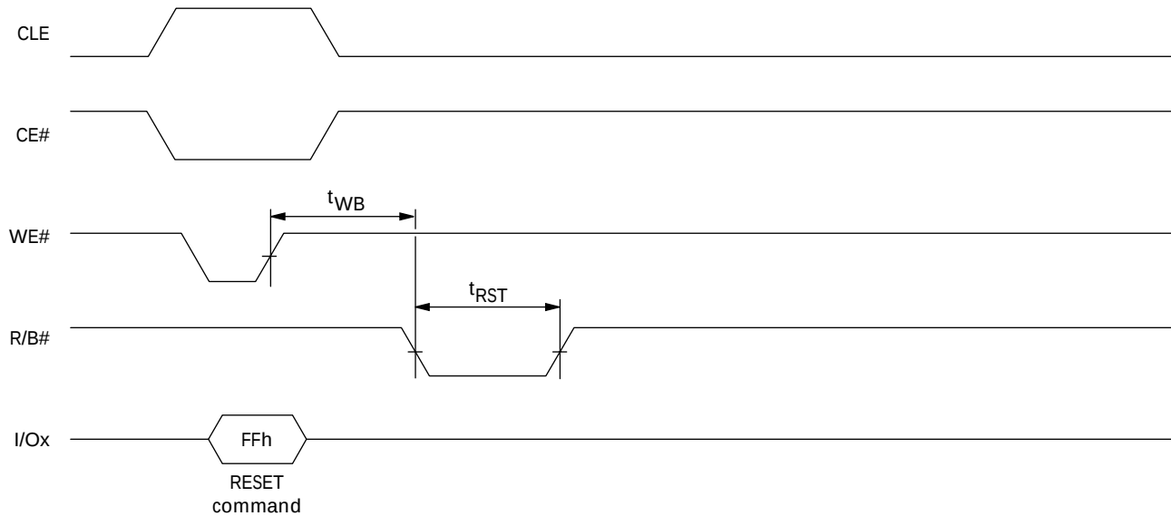
Figure 74: RESET Operation
