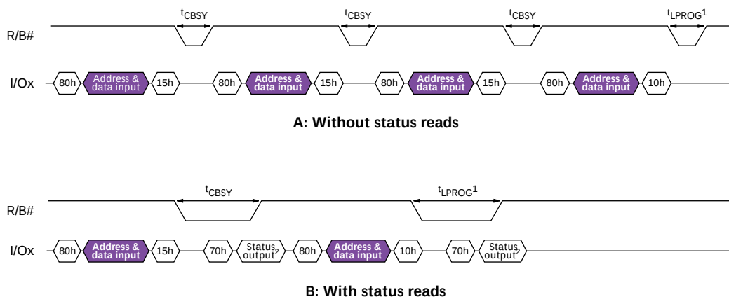
Figure 27: PROGRAM PAGE CACHE MODE Example
