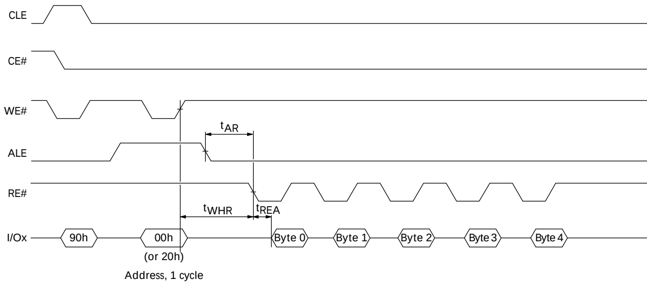
Figure 66: READ ID Operation
