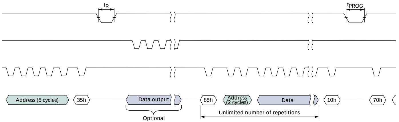
Figure 29: INTERNAL DATA MOVE with Optional RANDOM DATA Output and RANDOM DATA Input
