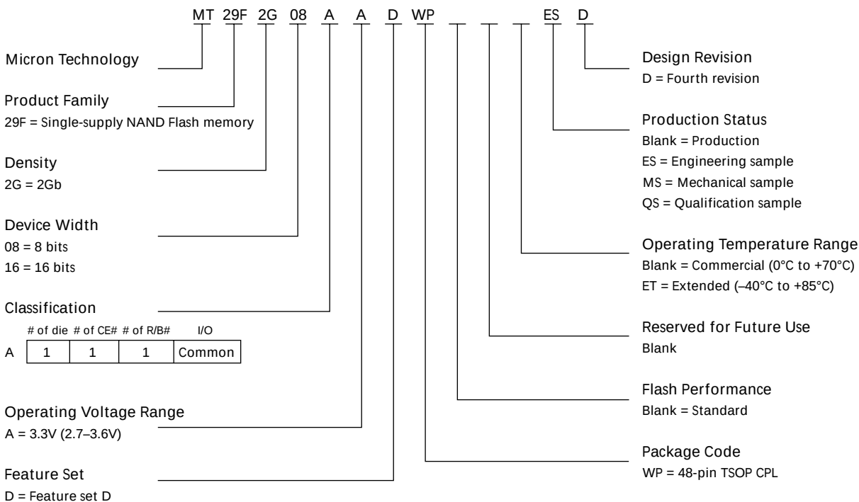
Figure 2: Part Number Chart (3.3V)
