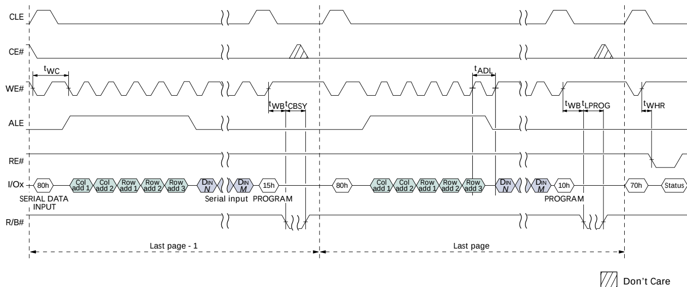
Figure 71: PROGRAM PAGE CACHE MODE Operation
