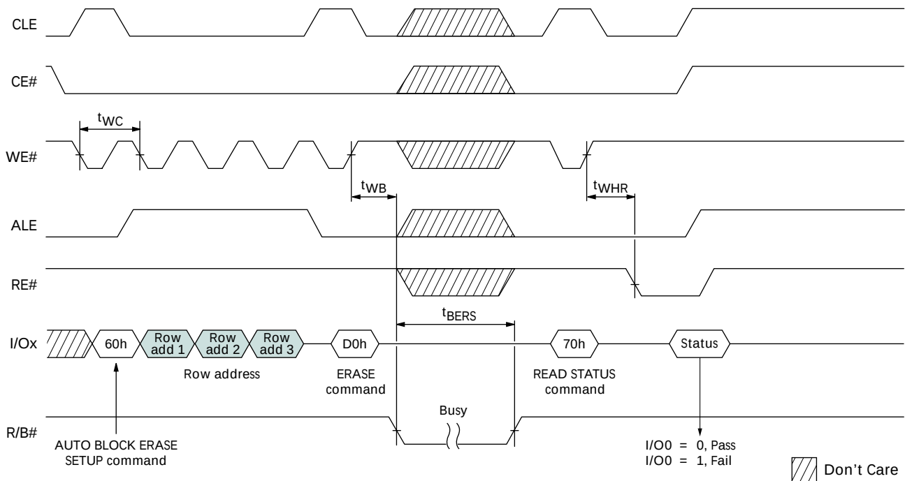
Figure 73: BLOCK ERASE Operation
