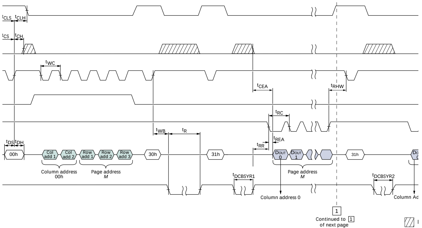
Figure 62: PAGE READ CACHE MODE Operation, Part 1 of 2
