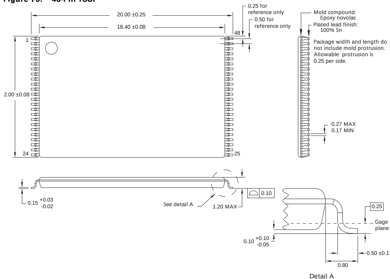
Figure 75: 48-Pin TSOP
