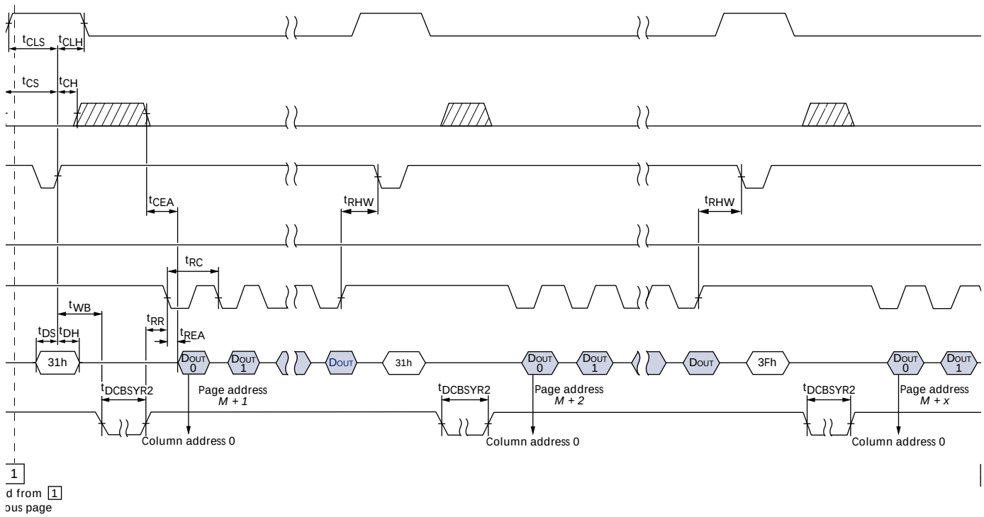
Figure 63: PAGE READ CACHE MODE Operation, Part 2 of 2
