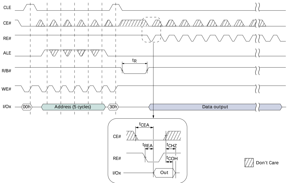
Figure 60: READ Operation with CE# "Don't Care"
