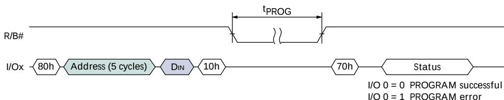
Figure 25: PROGRAM and READ STATUS Operation
