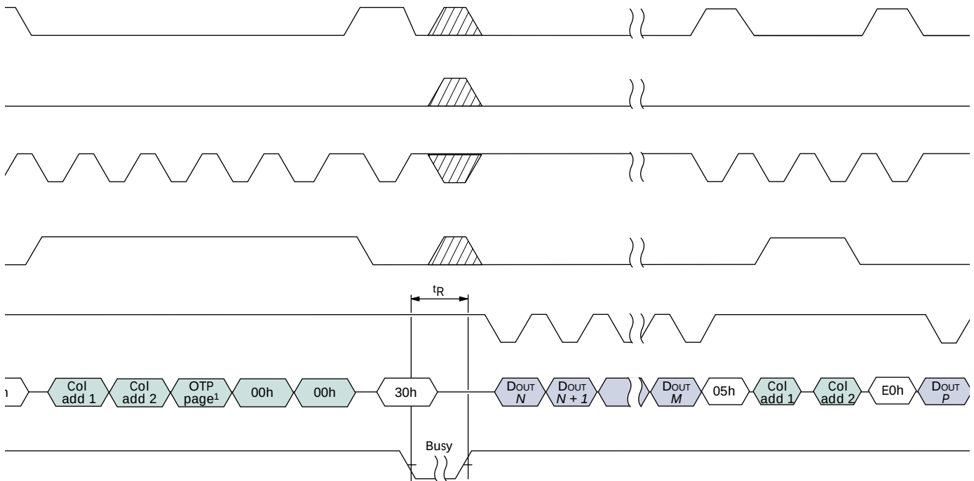
Figure 43: OTP DATA READ with RANDOM DATA READ
