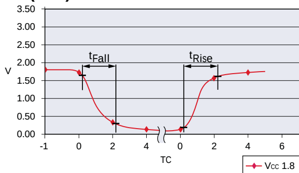
Figure 14: t_{Fall} and t_{Rise} (1.8V)
