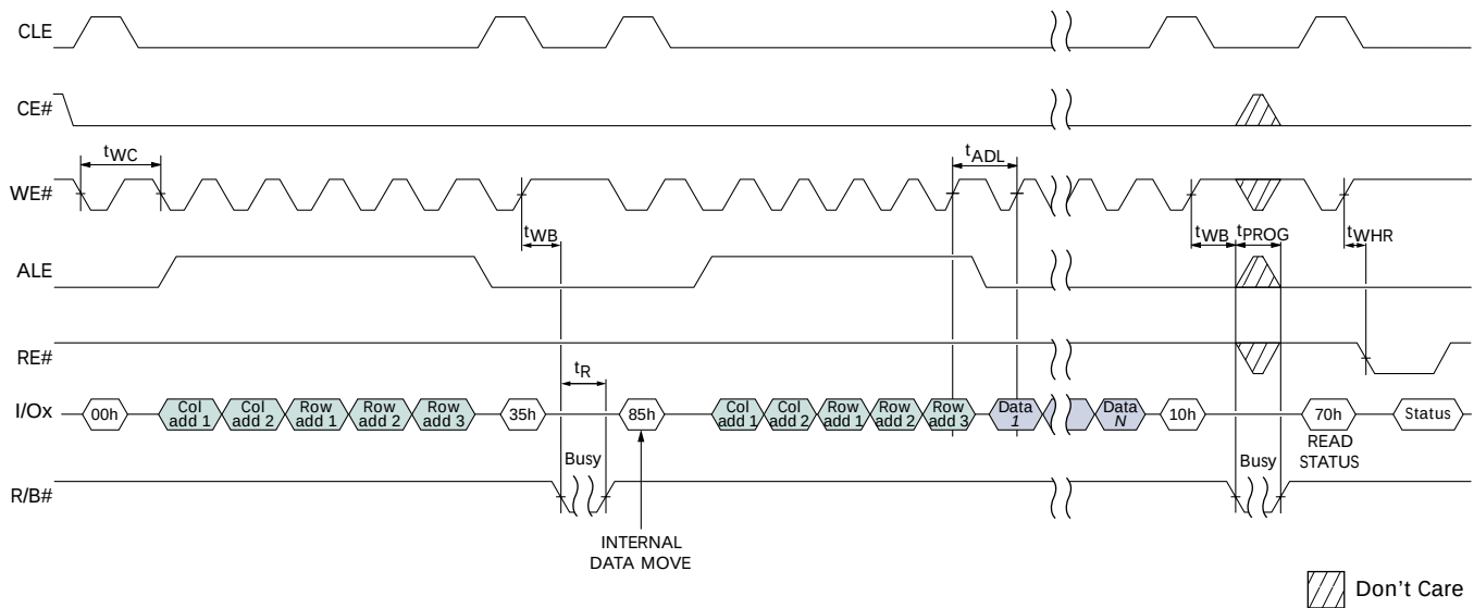
Figure 70: INTERNAL DATA MOVE Operation
