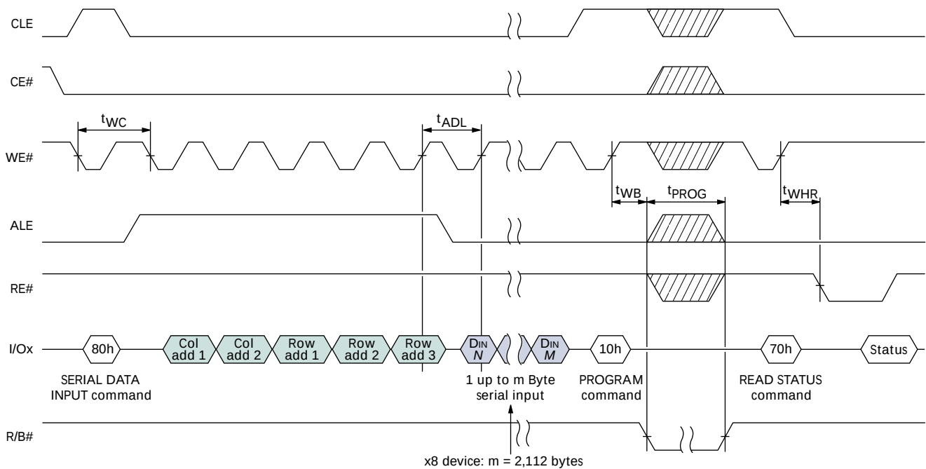
Figure 67: PROGRAM PAGE Operation
