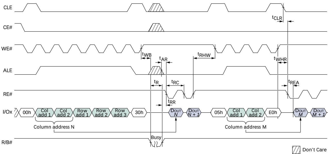
Figure 61: RANDOM DATA READ Operation
