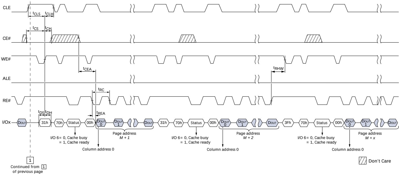
Figure 65: PAGE READ CACHE MODE Operation Without R/B#, Part 2 of 2
