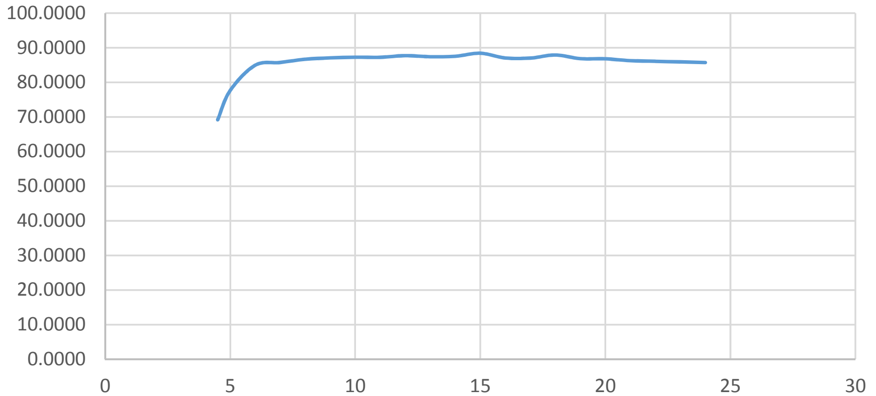
Efficiency at 5V @ 1.0 Amp
