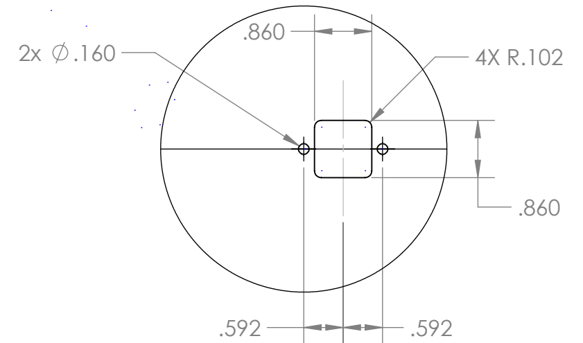
DETAIL B SCALE 1 : 2
