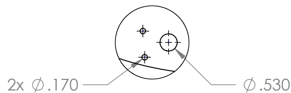
DETAIL F SCALE 1 : 3
