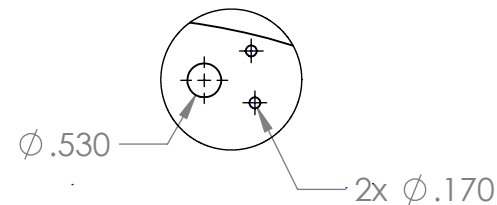
DETAIL E SCALE 1 : 3
