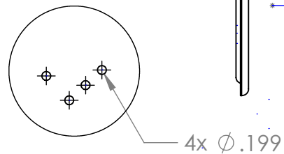
DETAIL D SCALE 1 : 3
