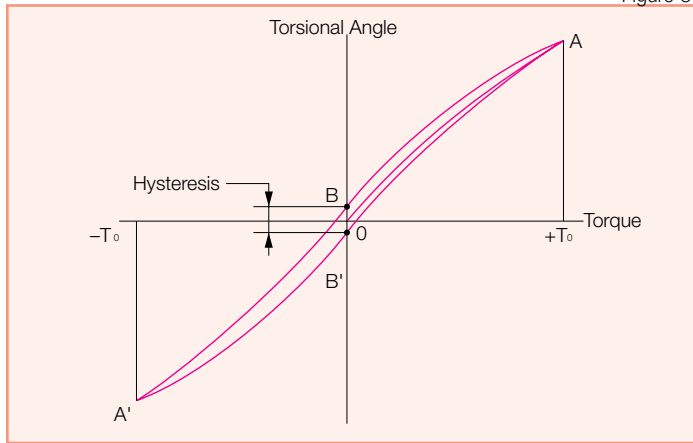
Torsional Stiffness for Ratio 1/30
