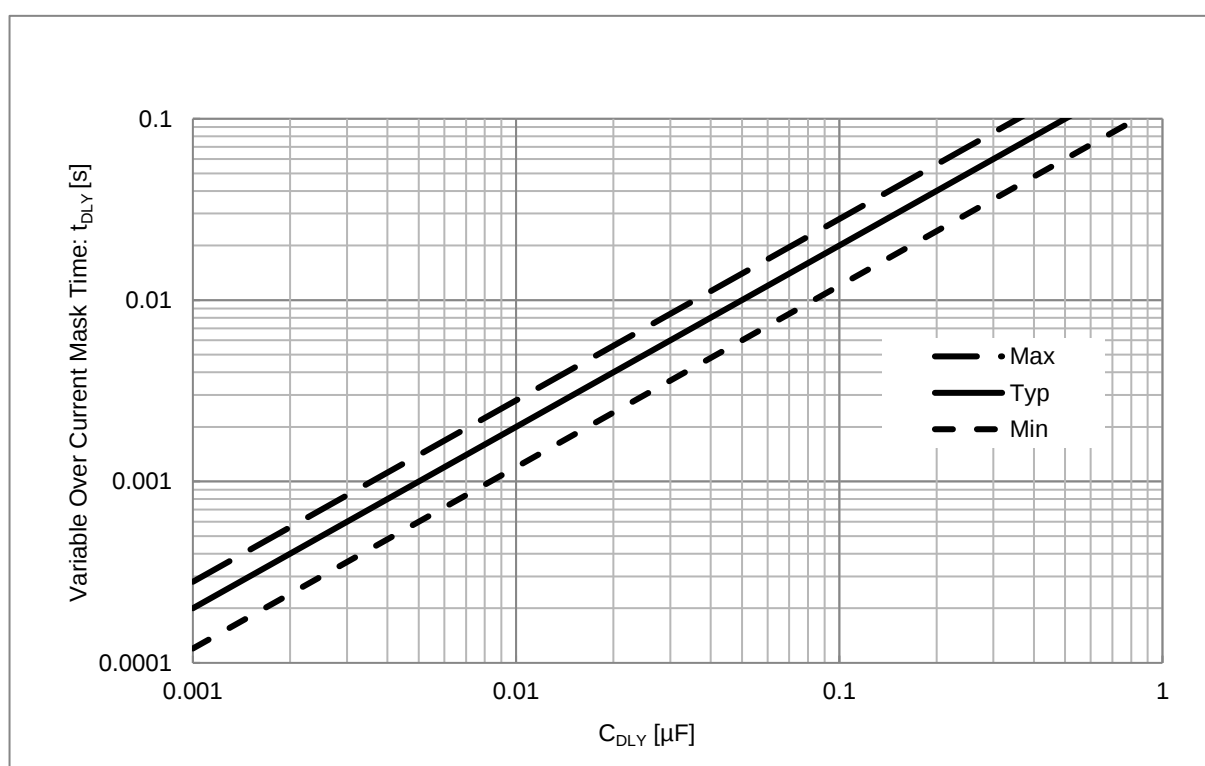
Figure 37. Variable Over Current Mask Time vs C_{DLY}
