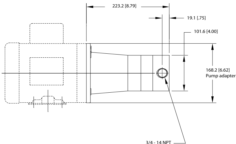
GN SERIES on NEMA MOUNT
