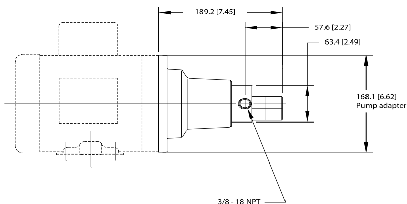
GK SERIES on NEMA MOUNT
