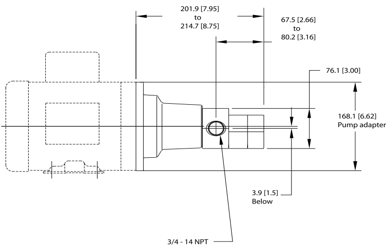
GL SERIES on NEMA MOUNT
