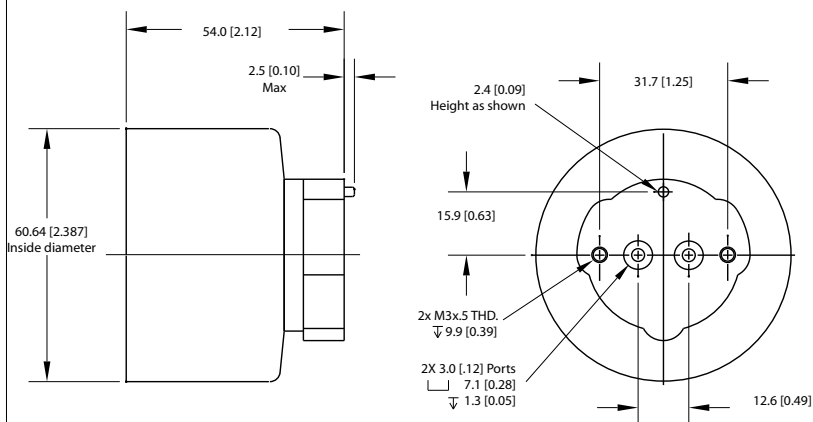
GAP SERIES on A MOUNT
