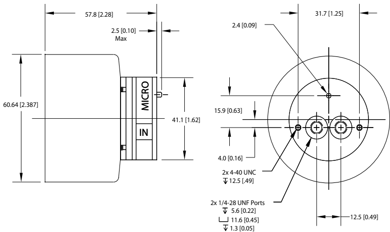
GAT SERIES on A MOUNT
