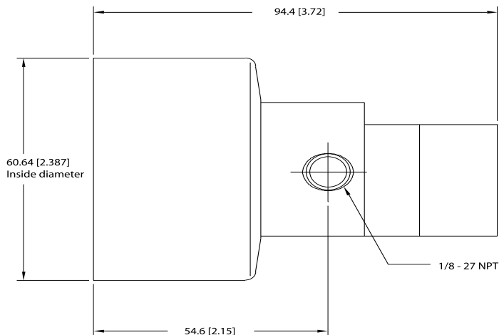
GJ SERIES on A MOUNT
