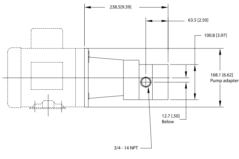
GM SERIES on NEMA MOUNT
