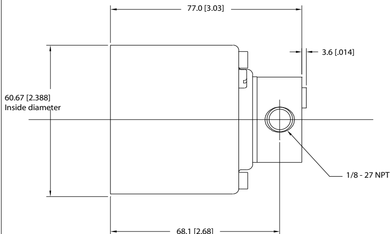
GB SERIES on A MOUNT
