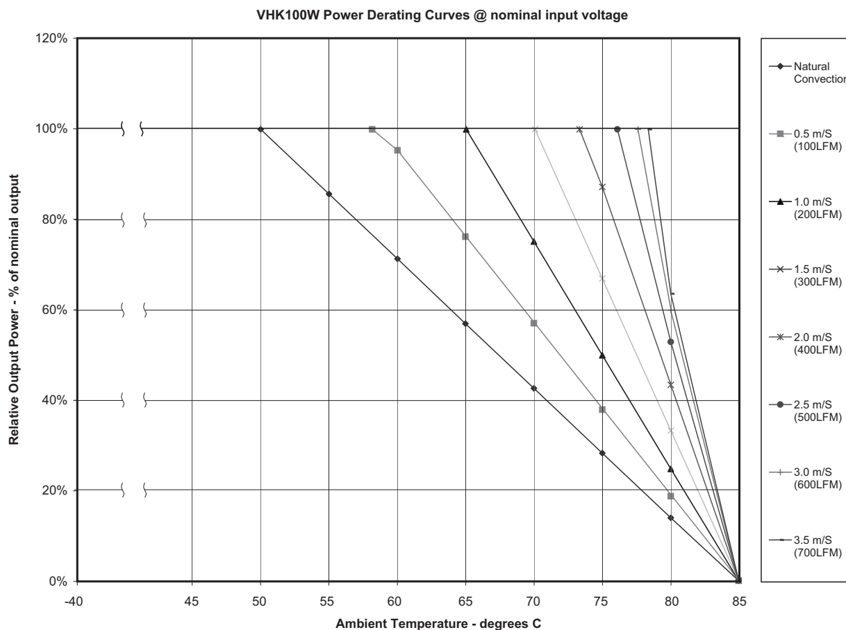
FIGURE 1. OUTPUT DERATING
