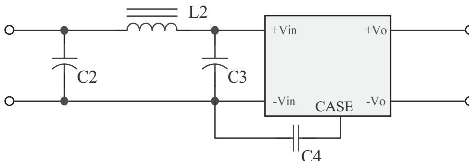
FIGURE 10. EMI FILTER FOR VHK75W
